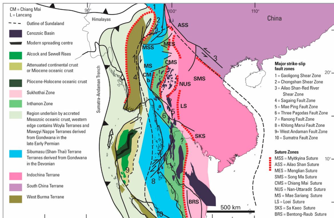
Figure 2. Tectonic map of SE Asia [25]. Cambodia is entirely contained within the Indochina terrain bounded on the northeast by the Song Ma Suture (SMS).
