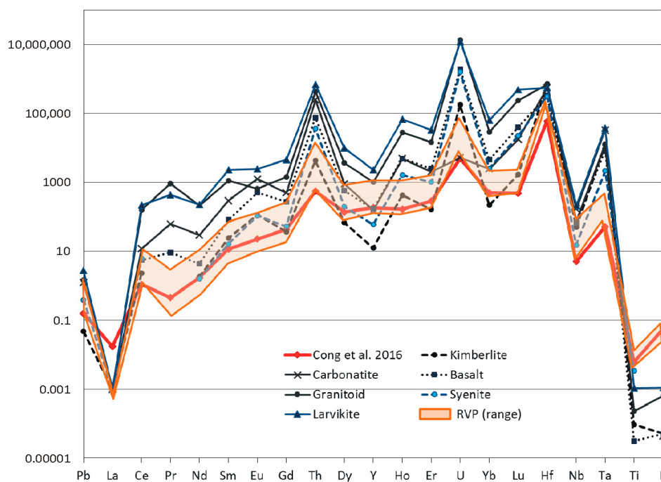
Figure 10. Chondrite-normalized trace element spidergram for zircon from the RVP (orange shaded region) including average data from Cong et al. (red [23]) and zircon from other rock types [5].
