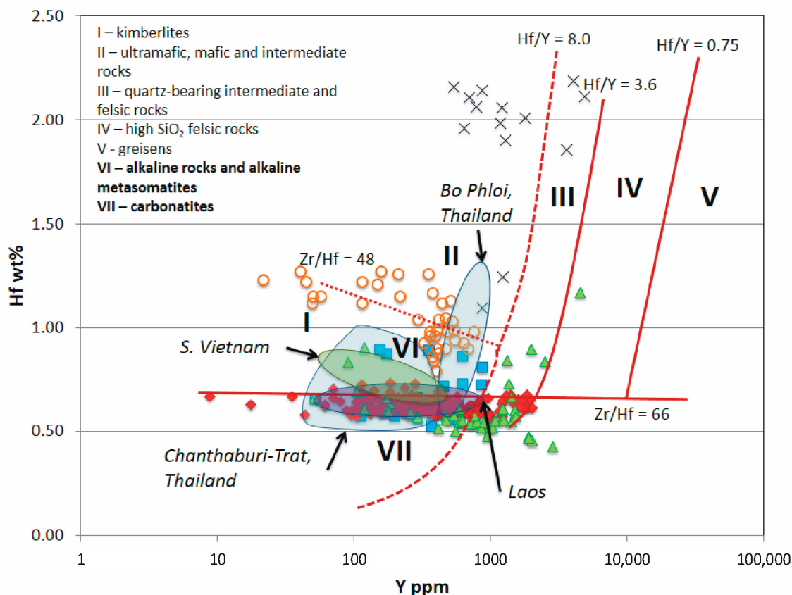
Figure 11. Y versus Hf discrimination diagram for RVP zircon, zircon xenocrysts from ZIP localities, and zircon inclusions in corundum (modified after [92]). Red diamonds: RVP zircon, blue squares: Pailin, Cambodia (Piilonen, unpublished data), blue field: Thailand (Piilonen, unpublished data), green triangles: Australia [11], orange circles: zircon xenocrysts from carbonatites [5], black crosses: zircon inclusions in corundum xenocrysts [10,12,38,97].
