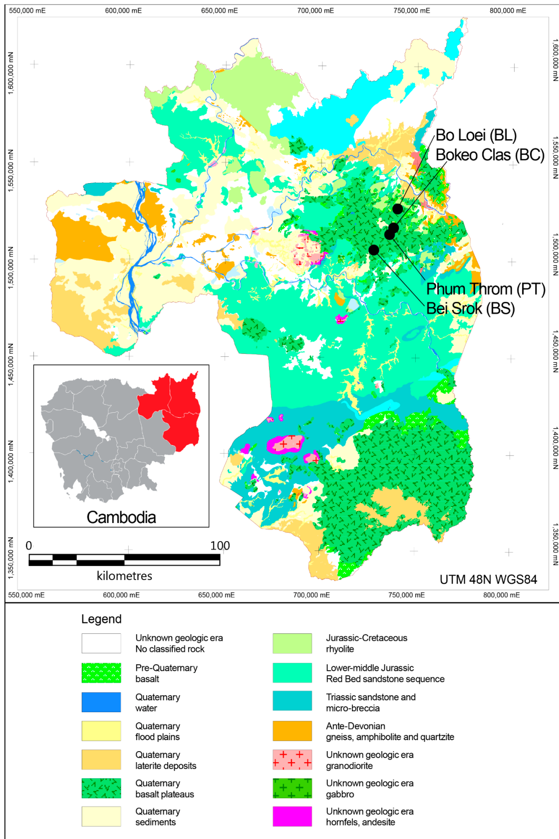
Figure 4. Geological map of Stung Treng, Ratanakiri, and Mondulakiri provinces, Northeast Cambodia. The Ratanakiri Volcanic Province (RVP) and Ban Chay Plateau Quaternary basalts are indicated in green with hatching. Zircon xenocryst localities (black dots) include Bokeo Clas (BC), Phum Throm (PT), Bei Srok (BS), and Bo Loei (BL).
