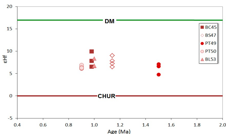
Figure 13. U-Pb Age (Ma) versus \epsilon_{\text{Hf}} for RVP zircon. CHUR: Chondritic uniform reservoir, DM: Depleted mantle.
