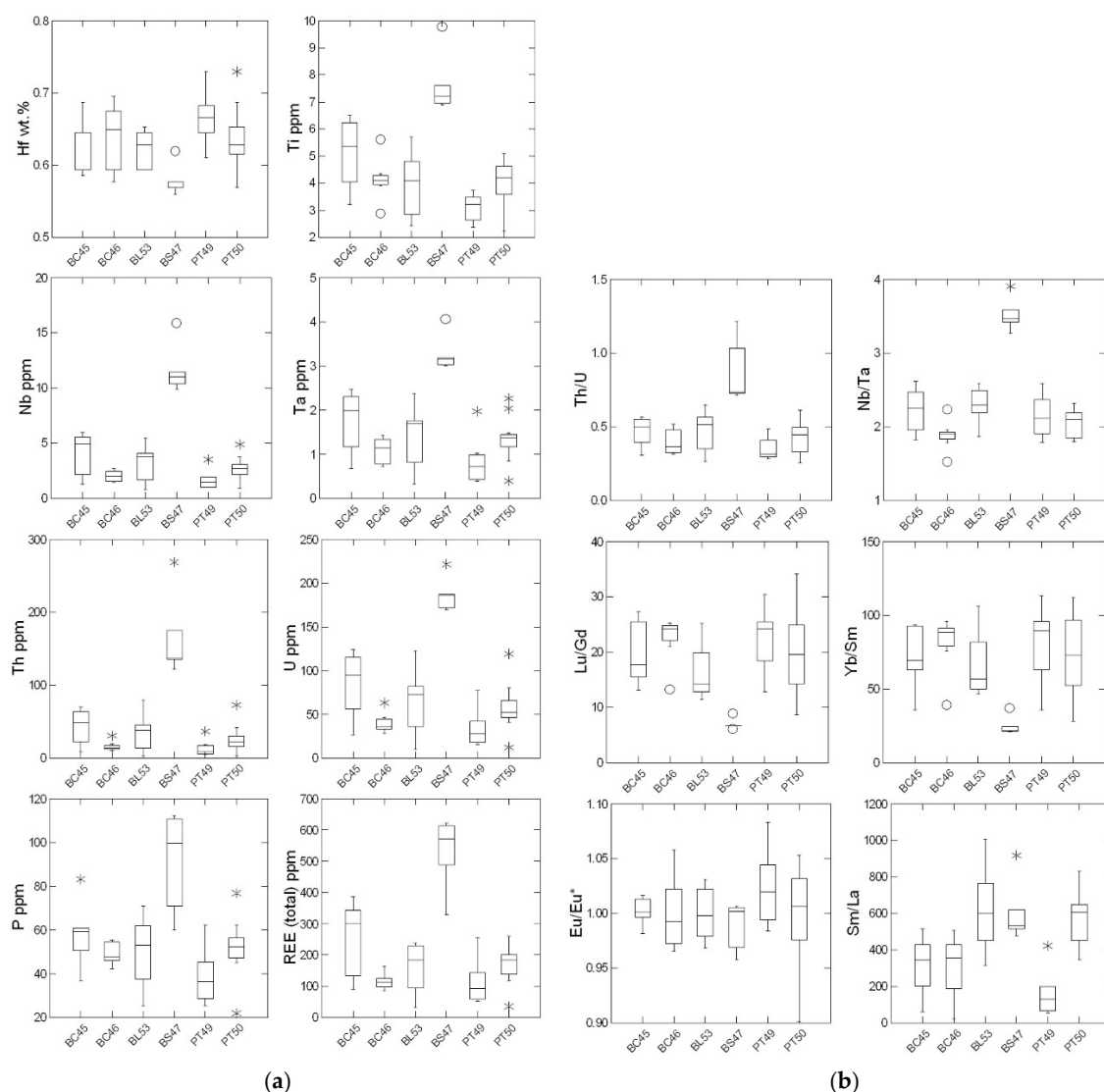
Figure 8. Boxplot diagrams for relevant trace element (a) and trace element ratios (b) in RVP zircon xenocrysts. The vertical line and whiskers represent the range in the data values with the horizontal line representing the median of the data set. The box is defined by the first and third quartiles.
