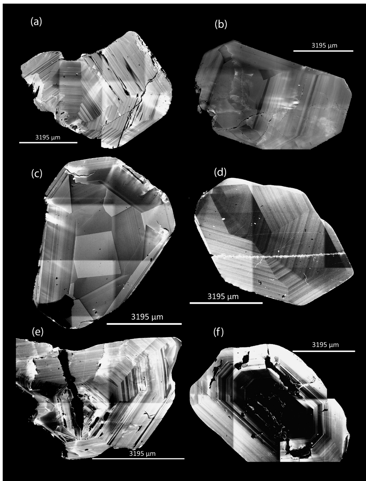
Figure 7. Cathodoluminescence images of RVP zircon xenocrysts showing both oscillatory and sector zoning. Darker zones are enriched in Th, U, and REE: (a) concentric zoning in BC43-2, (b) concentric zoning in PT49-2, (c) sector zoning in PT48-3, (d) sector and concentric zoning in BL54-3, (e) sector and concentric zoning in BL53-2, and (f) dark, CL-inactive core in BL53-1.
