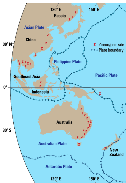
Figure 1. Map showing the 12,000 km long zircon megacryst Indo-Pacific zone (ZIP) along the western Pacific continental margins in Eastern Australasia, Asia, and Russia. The intraplate basalts hosting the megacryst suites are dominantly alkaline in composition and involve deeper mantle generation of magmas that may intersect pre-existing gem-bearing felsic or metamorphic bodies [11]. Consult this reference for zircon locality details.
