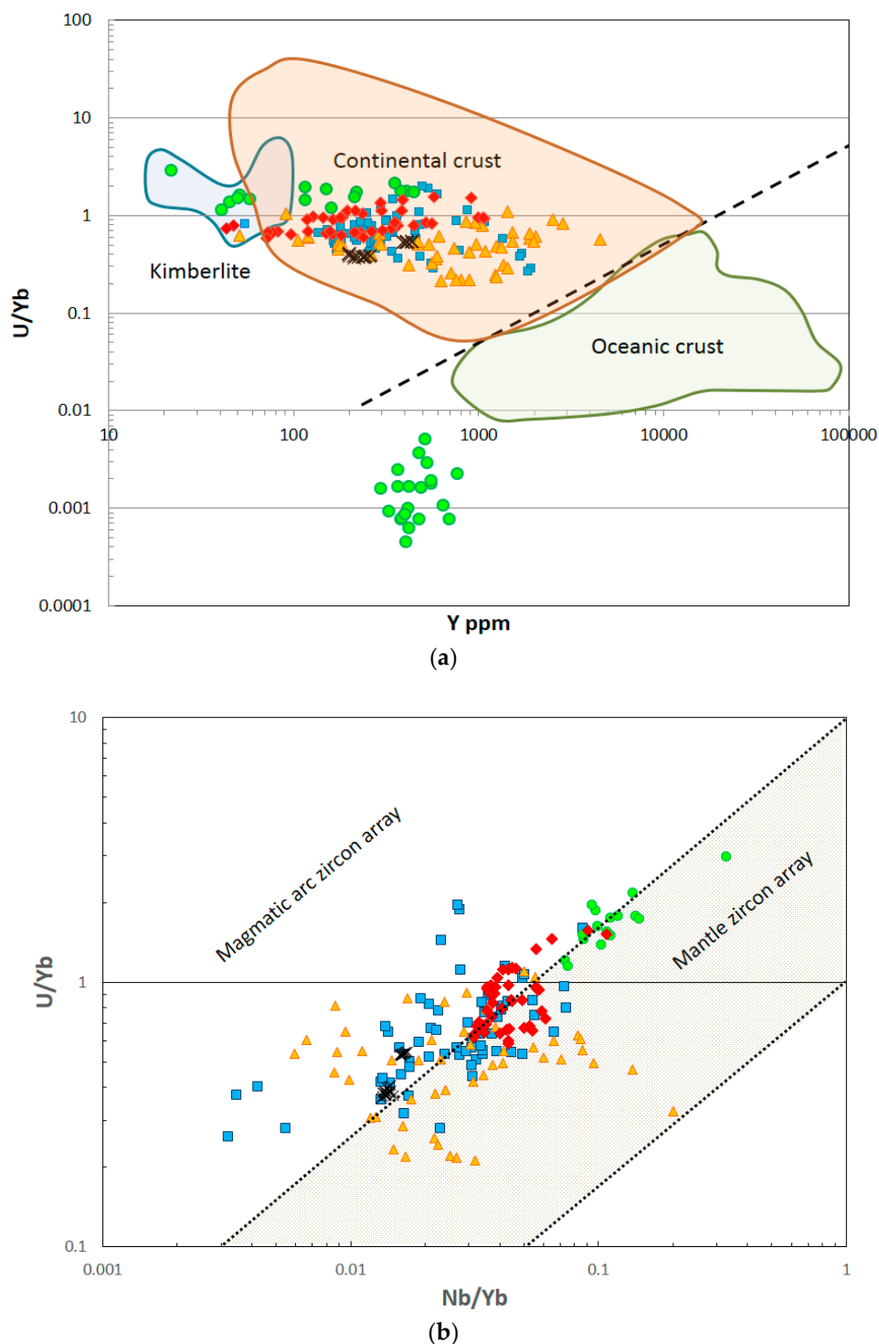
Figure 12. Y versus U/Yb (a) and Nb/Yb versus U/Yb. (b) Discrimination diagrams for zircon from the RVP (red diamonds, black X's [23]), Thailand (blue squares, Piiilonen, unpublished data), other ZIP localities (orange triangles, Australia, Laos, Vietnam [11]), and carbonatites (green circles [5]). Fields for continental and oceanic crust and kimberlite from Grimes et al. [105]. Fields for mantle and magmatic arc arrays from Grimes et al. [106].
