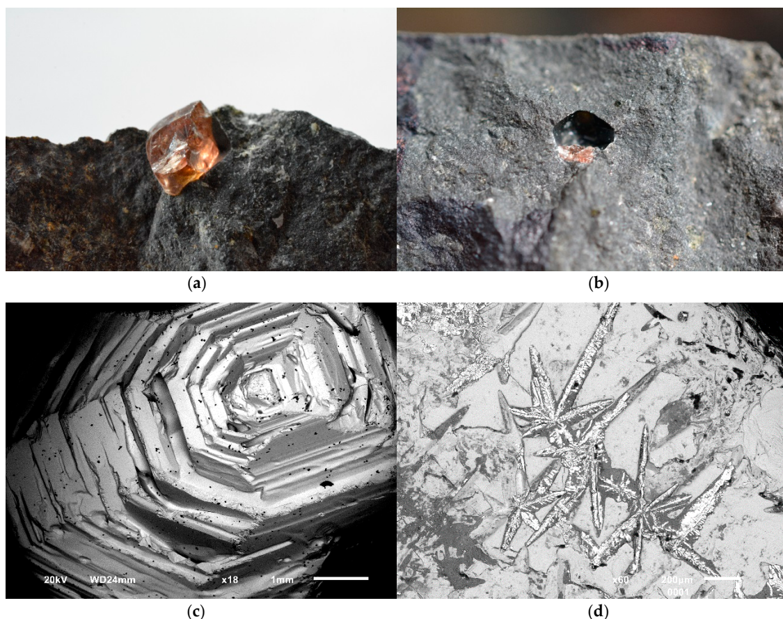
Figure 6. Zircon xenocrysts from the RVP: (a) euhedral zircon ( 7 \times 4.5 \times 4 mm) in situ from Phnom Dang, Bokeo. (b) Glassy reaction rim (1–2 \mu\text{m} wide lining the 5 mm hole) between zircon xenocryst and the host alkali basalt. (c) Hopper-type growth feature on the subhedral zircon. (d) Late-stage dendritic etching in-filled by baddeleyite on the surface of a zircon xenocryst.
