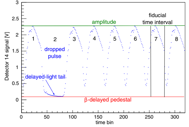
FIG. 2. Plot of a typical detector voltage signal as a function of time bin for eight 60 Hz neutron pulses. The proton pulse was not delivered to the spallation target in the 2nd pulse resulting in a dropped pulse. The peak yield in the 3rd pulse is 1% low because the phosphorescence tail from the second pulse is missing. The rising (falling) edges of the pulses correspond to the choppers opening (closing). The pedestal from the \beta -delayed \gamma 's of ^{28}\text{Al} is shown. Finally, the fiducial time interval (27 time bins wide) is shown in pulse seven (time bins 253 to 279).
