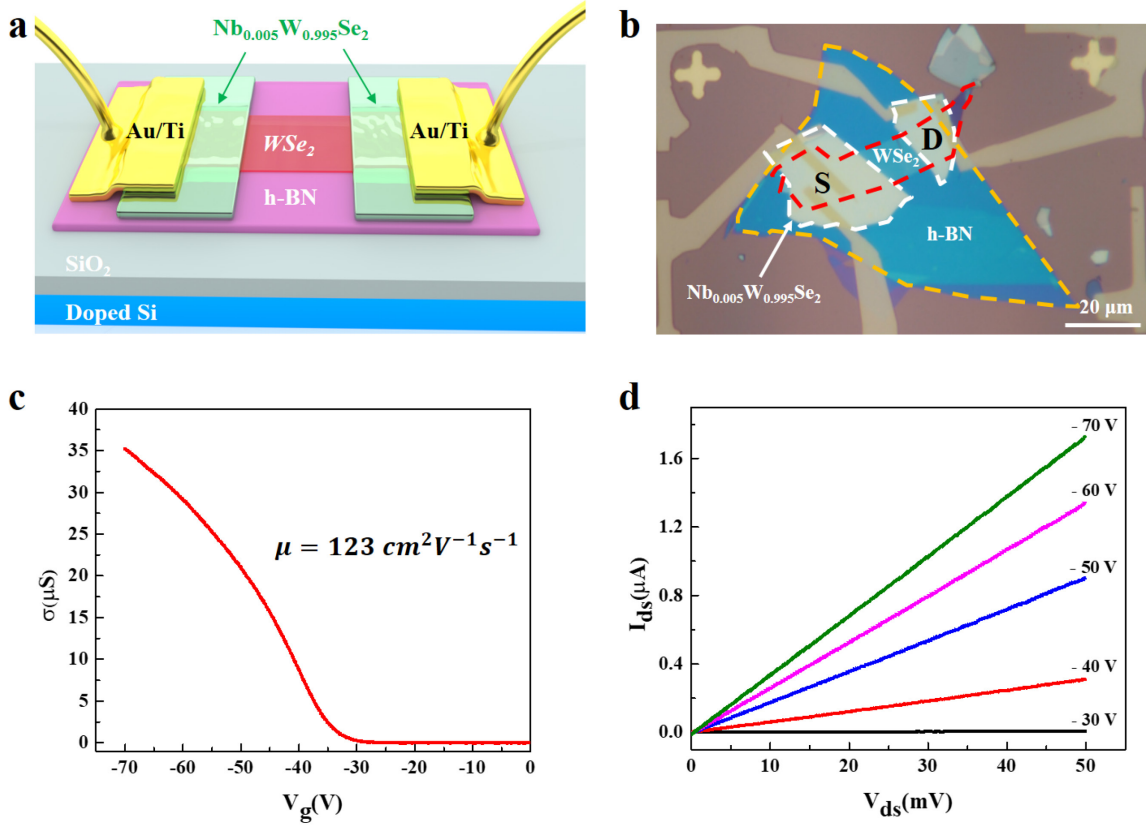
Figure 1. Configuration and characteristics of a WSe 2 FET with 2D/2D contacts. (a) Perspective side view of a WSe 2 FET with degenerately p-doped WSe 2 (Nb 0.005 W 0.995 Se 2 ) contacts. (b) Optical image of the device. The gold dashed line outlines the h-BN thin film. The white and red dashed lines represent the outlines of the Nb-doped WSe 2 contacts and undoped WSe 2 channel, respectively. (c) Modulation of the source-drain conductance by the back-gate voltage ( V_g ) at 77 K. (d) Linearity of the I_{ds} – V_{ds} characteristics indicating ohmic behaviors for a wide range of back-gate voltages.
