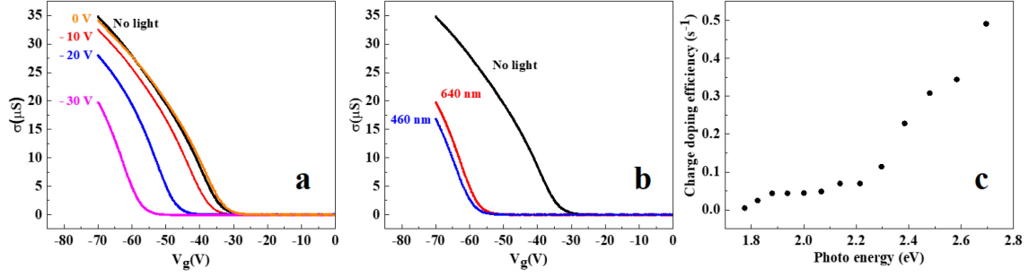
Figure 2. Experimental observation of the photo-induced doping in the WSe 2 FET. (a) Transport curves after 460 nm ( \sim 0.01 \mu W/\mu m^2 ) illumination with different back-gate voltages: V_g^{light} = 0V, -10V, -20V , and -30V , respectively. (b) Transport curves after 460 nm and 640 nm illumination with V_g^{light} = -30V . (c) Photo-induced doping efficiency as a function of photon energy with V_g^{light} = -50V .
