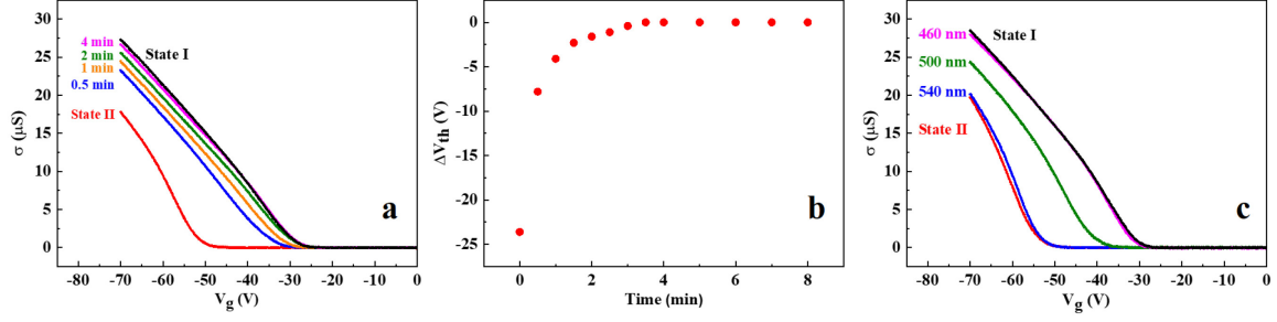
Figure 4. The comparison of the restoring process in WSe 2 /h-BN heterostructures under illumination with different wavelengths. (a) State I and State II represent the response of the device before and after 460 nm illumination with V_g^{light} = -30 V, respectively. (b) The restoring process under 460 nm illumination with V_g^{light} = 0 V. \Delta V_{th} denotes the threshold voltage ( V_{th} ) shift of the device compared to that of State I. (c) During the restoring process, the device is tested with a back-gate voltage of V_g^{light} = 0 V under 540 nm, 500 nm and 460 nm illumination, respectively.
