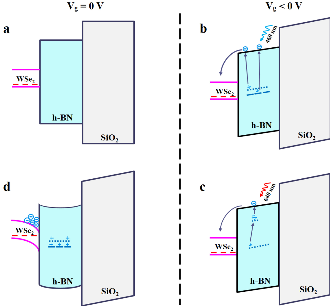
Figure 3. Photo-induced doping mechanisms for WSe 2 FETs on h-BN substrates. The red dash lines correspond to the Fermi level of the undoped WSe 2 channel. Blue dashed and dotted lines represent V_N and N_B V_N defect states in h-BN substrates, respectively. (a) The band diagram of the WSe 2 FET under equilibrium conditions ( V_g = 0 V). The band diagrams of the WSe 2 FET with V_g^{light} < 0 V under (b) 460 nm and (c) 640 nm illumination, respectively. (d) The band diagram of the photo-doped WSe 2 FET after the doping process is completed with V_g = 0 V.
