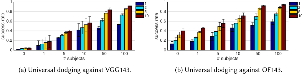
Fig. 7. Universal dodging against VGG143 and OF143. The x-axis shows the number of subjects used to train the adversarial generators. When the number of subjects is zero, a non-adversarial generator was used. The y-axis shows the mean fraction of images misclassified (i.e., the dodging success rate). The whiskers on the bars show the standard deviation of the success rate, computed by repeating each experiment five times, each time with a different set of randomly picked subjects. The color of the bars denotes the number of eyeglasses used, as shown in the legend. We evaluated each attack using 1, 2, 5, or 10 eyeglasses. For example, the rightmost bar in Figure 7(b) indicates that an AGN trained with images of 100 subjects will generate eyeglasses such that 10 pairs of eyeglasses will allow approximately 94% of subjects to evade recognition. For \leq 10 subjects, Algorithm 1 was used to create the attacks. For 50 and 100 subjects, Algorithm 2 was used.
