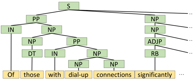
Figure 5. The phrase tree generated by the Stanford CoreNLP constituency parser for the sentence “Of those with dial-up connections, significantly more men than women said they were interested in high-speed connections”. Each subtree indicates a phrase and our syntactic matching algorithm finds a match between the phrase ‘dial-up connections’ and a cell in the table of Figure 1(right).
