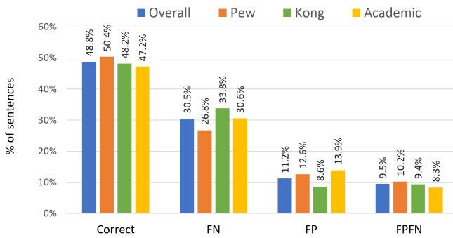
Figure 10. Comparison of correct, FN, FP and FPFN references produced by our complete pipeline for each of the datasets, Pew (orange), Kong (green) and Academic (yellow) as well as the overall combination of all three datasets (blue).
