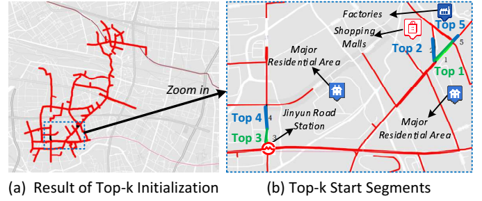
Fig. 7. Top- k Initialization Example.
