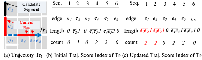
Fig. 11. Example of Efficient Trajectory Score Computing & Update.
