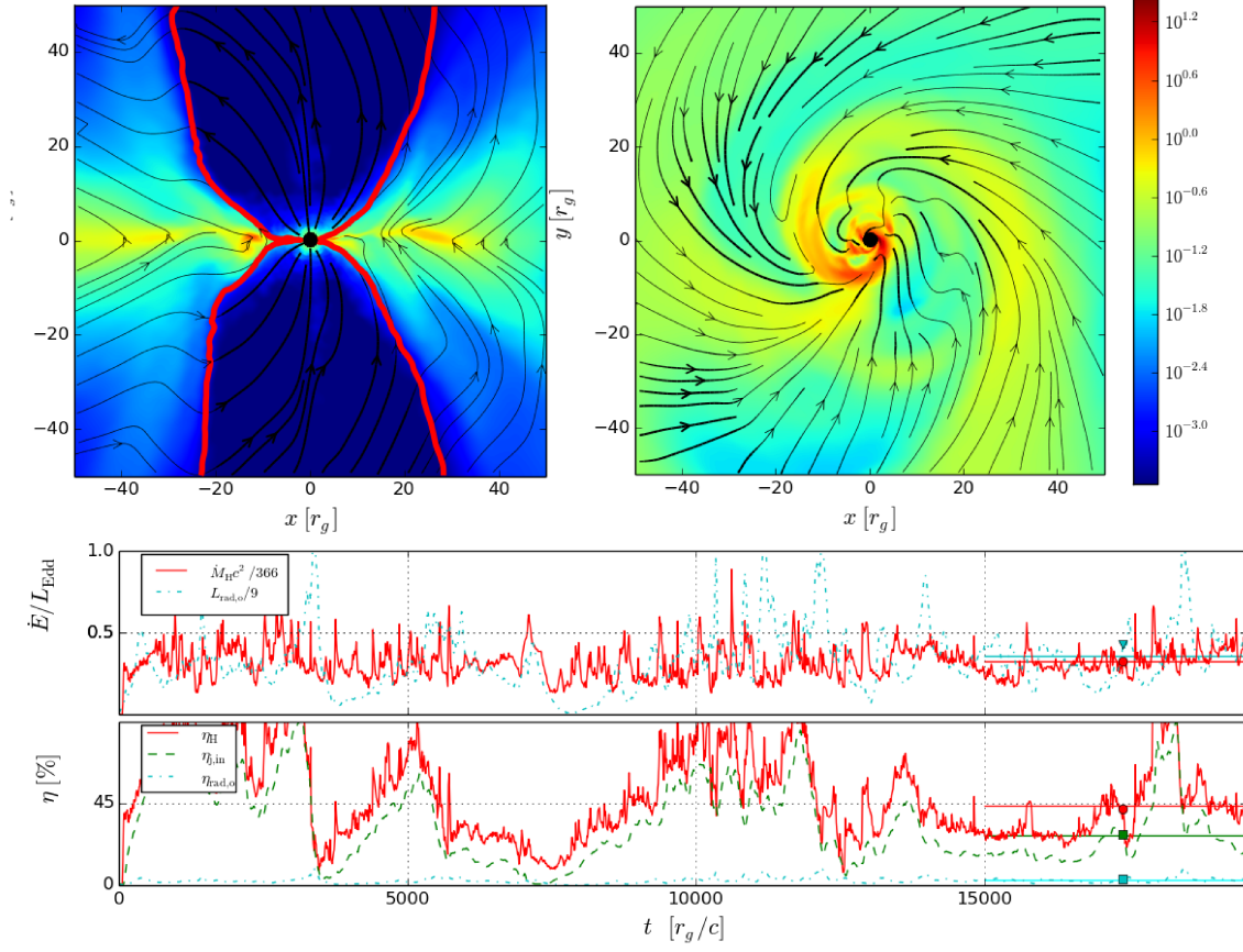
Figure 2. Evolved snapshot (at t = 17400 R_g/c ) showing \log_{10} of rest-mass density (scaled by an Eddington density of \rho_{\text{Edd}} = \dot{M}_{\text{Edd}}/(4 \pi/3 r_g^3) \sim 4 \times 10^{-12} \text{ g cm}^{-3} , shown in color with legend on right) in both the z-x plane (top-left panel) and y-x plane (top-right panel). Black lines trace field lines, where thicker black lines show where field is lightly mass-loaded. In the top-left panel, the thick red line corresponds to the jet boundary where the electromagnetic energy equals the rest-mass energy of the gas. The bottom panel has two sub-panels. Horizontal solid lines show the averages over the period from 15000 R_g/c until the end of the simulation, while square/circle tickers are placed at the given time and values. The top sub-panel shows \dot{M} through the black hole horizon and radiative luminosity ( L_{\text{rad,o}} , from optically thin region at r \sim 1000 R_g ). All quantities have been normalized by the Eddington luminosity, where in addition the mass flux has been divided by \approx 366 and radiative luminosity by \approx 9 , so that both quantities can be shown on a single panel. The bottom sub-panel shows the efficiencies, where \eta_H is the total efficiency, \eta_{\text{j, in}} is the jet efficiency, and \eta_{\text{rad,o}} is the radiative efficiency.
