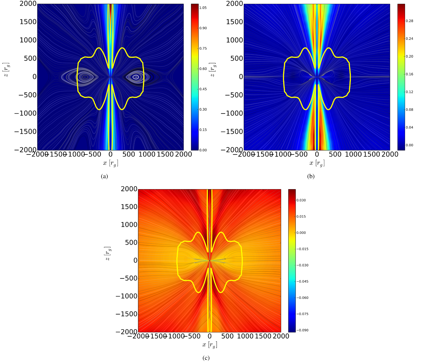
Figure 4. The left panel (a) shows time- \phi -averaged magnetic flux lines (translucent gray lines) with electromagnetic luminosity per unit angle (dL_{EM}/d\theta)/(\dot{M}_H c^2) \sim (dL_{EM}/d\theta)/(120 L_{Edd}) (color with legend), with blue contour showing the jet boundary, and yellow contour showing the electron scattering photosphere. The image is duplicated across the x = 0 line. The middle panel (b) shows the gas velocity flux lines and kinetic + gravitational energy luminosity per unit angle. The outflows wrap around the compact disk. The right panel (c) shows the lab-frame radiation flux lines and radiation luminosity per unit angle. Most of the kinetic energy escapes through the funnel region, carried by strong outflows. The radiation flux leaked through this region can also be super-Eddington, as compared to being Eddington-limited at other inclination angles.
