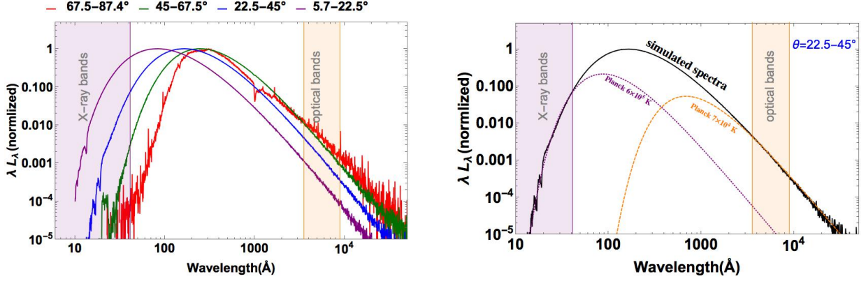
Figure 5. (a) The simulated escaping spectra from inclination angles bin 1 (red curve, closest to mid-plane) to bin 4 (purple curve, closest to the pole). The optical to X-ray ratio increases with inclination angle. The purple shaded region corresponds to X-ray band with energy below 0.3 keV. The orange shaded region corresponds to the optical band from 3560Å to 9000Å. (b) The simulated escaping spectrum (black curve) from intermediate angle bin 3, the shapes of which is broader than a blackbody spectrum. We also show two Planck functions, one fitting the X-ray continuum component (purple dotted curve) and the other one fitting the optical continuum component (orange dashed curve).
