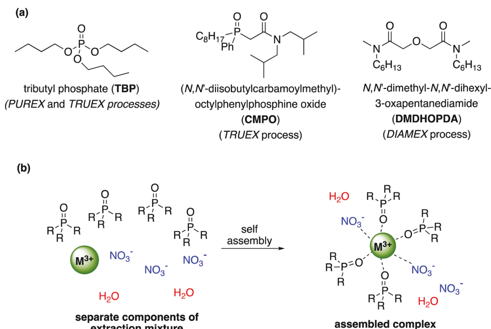
Fig. 2 (a) Structures of organic ligands used in the PUREX, TRUEX and DIAMEX solvent extraction processes; (b) depiction of the assembly process that occurs during a liquid–liquid extraction protocol.
