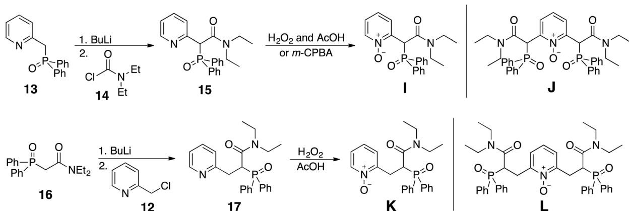
Fig. 8 Synthesis of CMPO substituted pyridine- N -oxide derivatives I–L .
