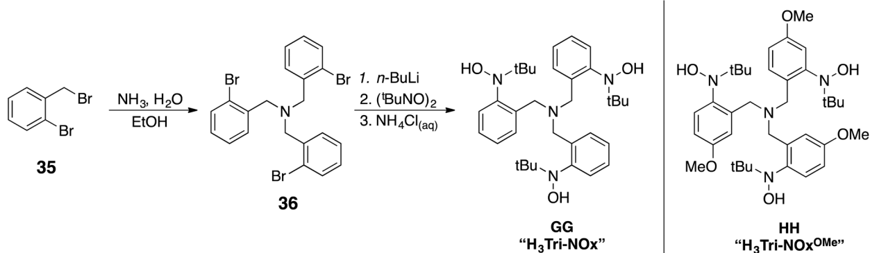
Fig. 15 Synthesis of tripodal TriNOx ligands GG and HH .
