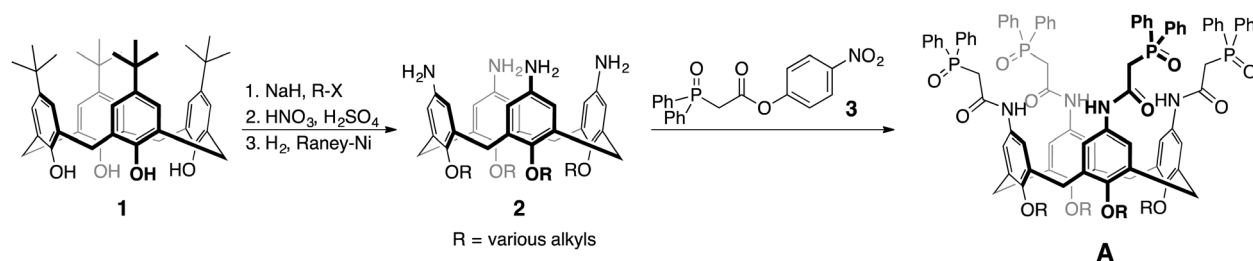
Fig. 3 Synthetic approach to wide-rim CMPO-substituted calix[4]arenes.
