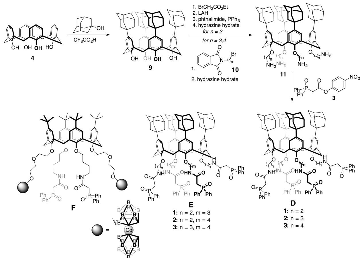
Fig. 6 Synthesis of substituted calixarenes D, E and F bearing CMPO groups at the narrow rim.
