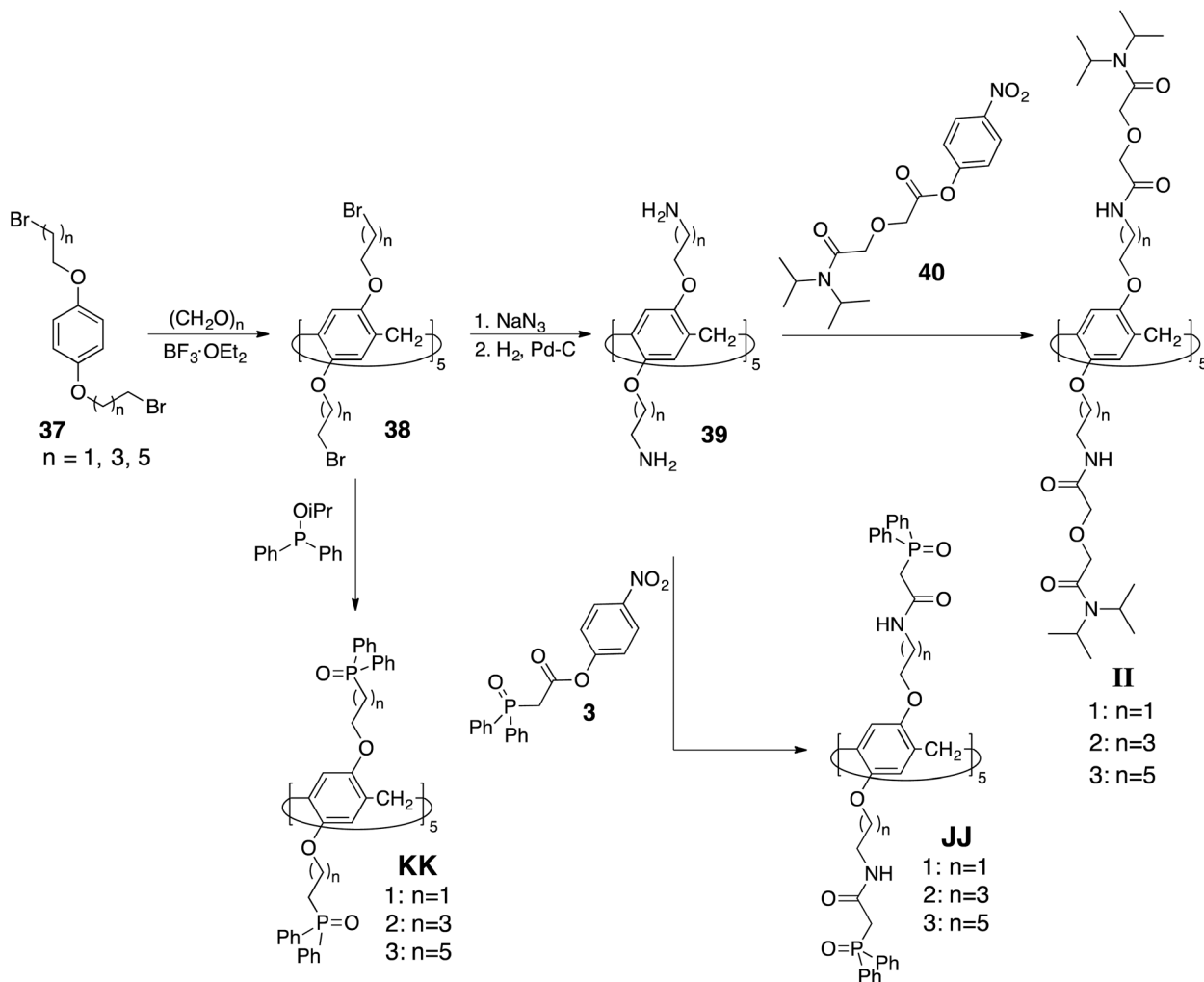
Fig. 16 Synthesis of pillar[5]arene compounds II, JJ and KK.
