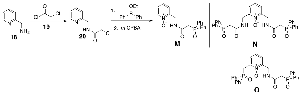
Fig. 9 Synthesis of pyridine- N -oxide derivatives M–O .
