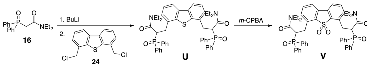
Fig. 11 Synthesis of CMPO-substituted dibenzothiophene and dibenzosulfone ligands U and V.
