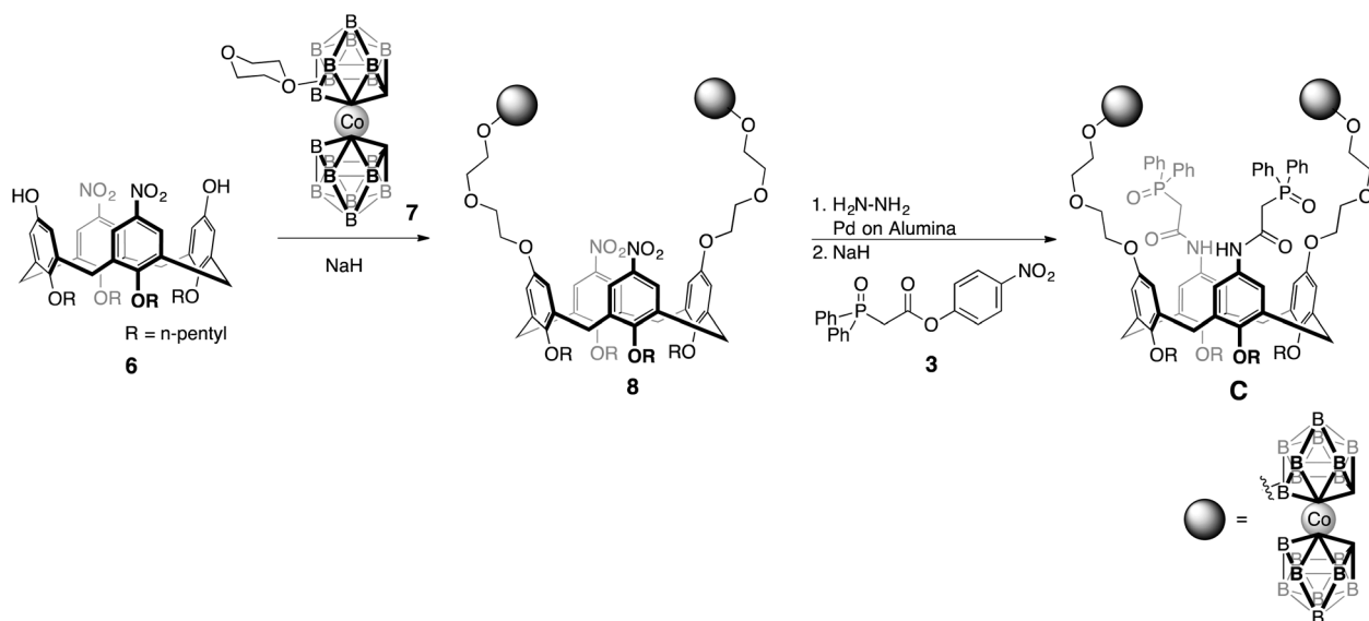
Fig. 5 Synthesis of anionic bis(dicarbollide)-substituted calix[4]arene C.
