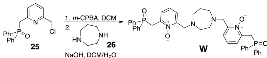
Fig. 12 Synthesis of 1,4-diazepane derivative W.
