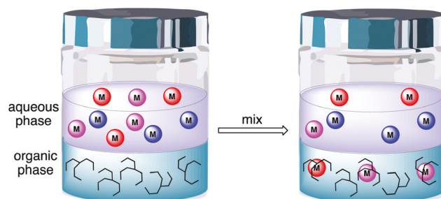
Fig. 1 Schematic representation of liquid-liquid extraction process for f-element separations. The colored spheres represent metal ions, dissolved initially in an acidic aqueous phase. Upon mixing, the chelating agent, represented by a generic line-angle structure, binds and extracts the metal ions into the organic layer in the form of metal-ligand complex.
