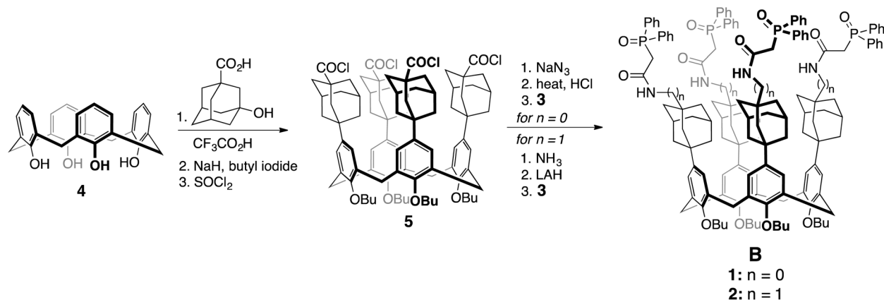
Fig. 4 Synthesis of adamantyl-linked CMPO calixarene derivatives B1 and B2.
