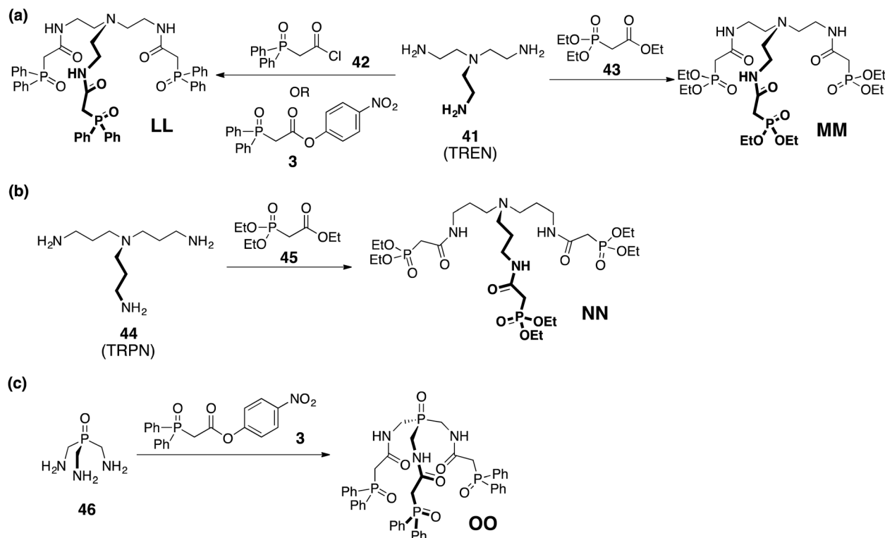
Fig. 17 Synthesis of a series of tripodal ligands, LL–OO, that present CMPO groups.
