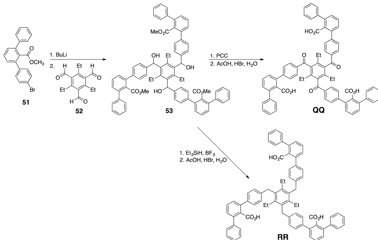
Fig. 19 Synthesis of two tripodal receptors QQ and RR .
