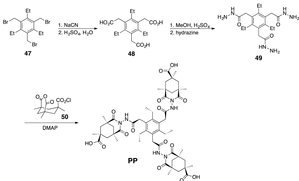
Fig. 18 Synthesis of supramolecular tricarboxylic acid ligand PP.
