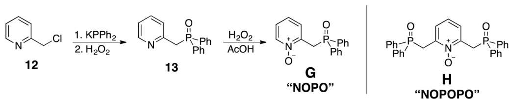
Fig. 7 Synthesis of pyridine- N -oxide derivatives "NOPO" (G) and "NOPOPO" (H).
