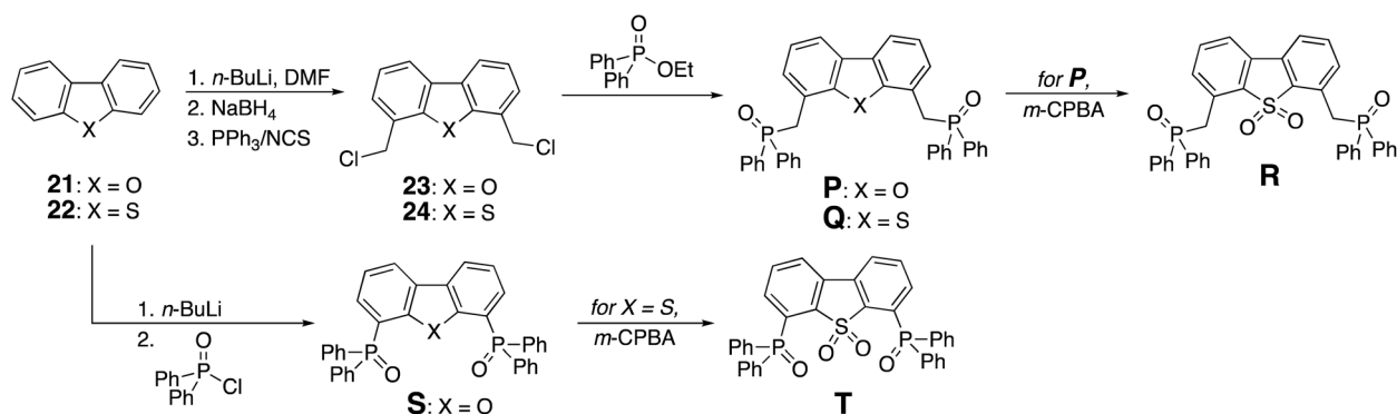
Fig. 10 Synthesis of dibenzofuran and dibenzosulfone ligands P–T.
