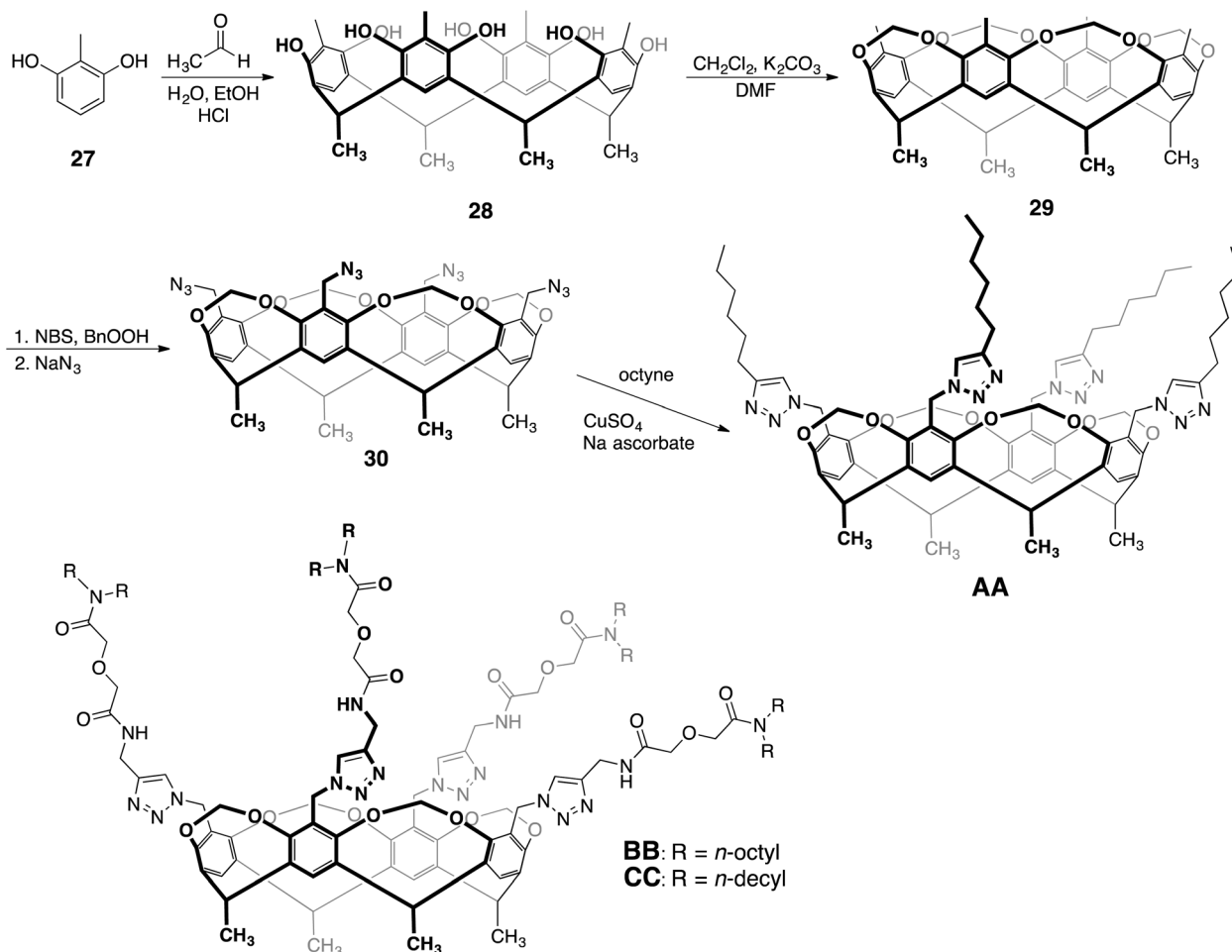
Fig. 13 Synthesis of diglycolamide-substituted cavitands AA–CC.
