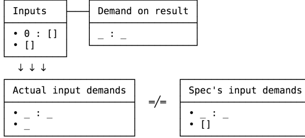
Fig. 4. Counterexample for rot_naive under rot_spec
