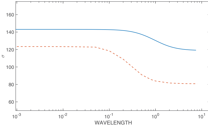
FIGURE 4. Solid curve is the dispersion coefficient \sigma versus \ell for the simplified model (see (4.4)) and dashed curve is the corresponding coefficient for the full model computed numerically. In both cases, \lambda_{t=0} = 0.05 , approximately the ‘edge’ of the faster growth plateau. Because the simplified model has increased biomass, its effective active layer is smaller (shifting the dispersion curve to the right) and growth is somewhat faster since effective flux of substrate into the biofilm layer is larger (shifting the dispersion curve upwards). Parameter values: Y = 1 , r_0 = 400 , c_0 = 1 , D^- = D^+ = 0.05 , H = 0.40625 , L = 0.09375 , \theta_0(0) = 0.05 .
