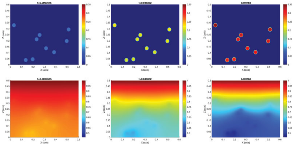
FIGURE 6. Time snapshots from a realisation of randomly but relatively sparsely embedded circular microcolonies. Top: biomaterial volume fraction at three successive times. Bottom: substrate concentration at the same three times.
