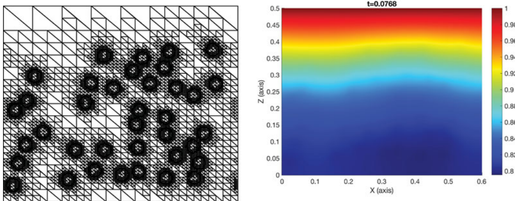
FIGURE 7. (Left) An example of a typical 1-irregular (i.e., at most one hanging node per element edge) adaptive mesh. Use of hanging nodes minimises mesh propagation. The mesh is obtained by successive refinement (using quadrisecion) and coarsening of an initial mesh containing only a few large triangles. The triangles are selected to be refined or coarsened according to a marking strategy described in [3] and references therein, based on inverse inequality estimates. The same number of boundary edges occur on opposing periodic domain sides as a result of the periodic mapping used. (Right) Computed substrate concentration using the same mesh.
