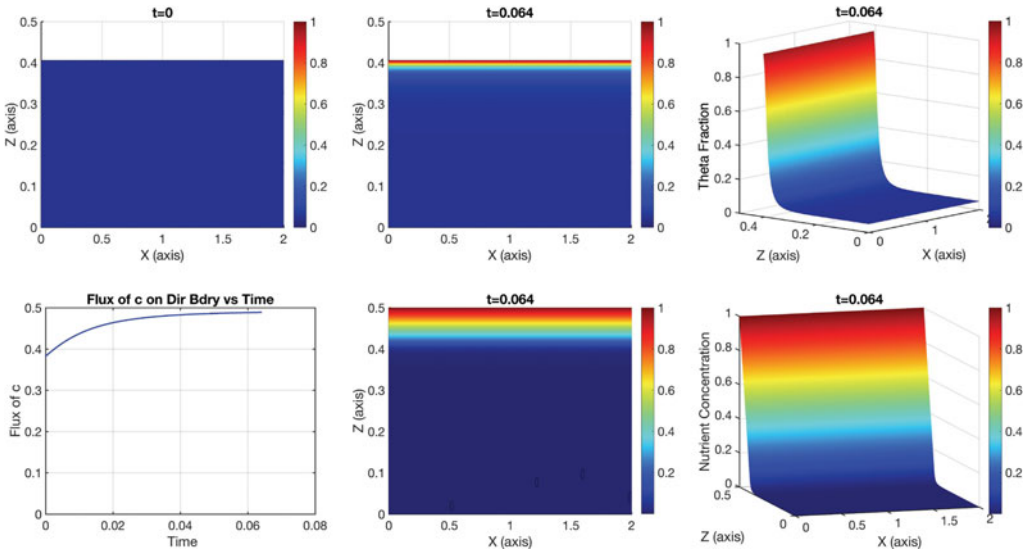
FIGURE 3. Example solution of (3.1)–(3.2). Top row: volume fraction \theta(z,t) with initial conditions (top left) \theta(z,0) = 0.05 . Bottom left: flux of c through the top of the biofilm-matrix region. Bottom middle, right: concentration c(z,t) . Parameters: r_{\max} = 720 , K = 0.8 , Y = 1 , D^+ = D^- = 0.05 , c_0 = 1 , H = 0.40625 , H + L = 0.5 .
