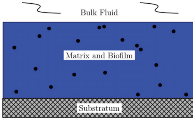
FIGURE 1. Internal micro-biofilms (black circles) included in a larger matrix.
