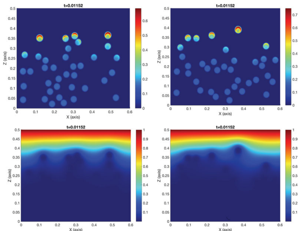
FIGURE 5. Two realisations of randomly embedded circular microcolonies. Top: biomaterial volume fraction. Bottom: substrate concentration.
