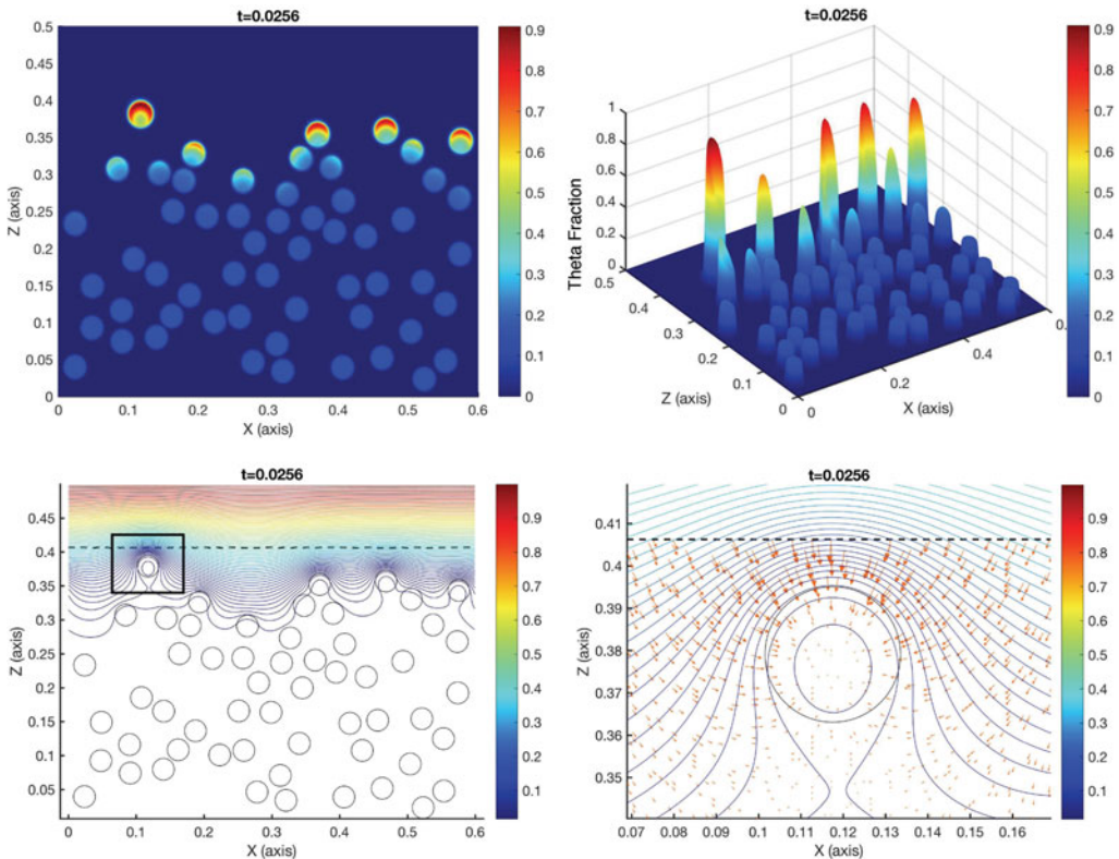
FIGURE 2. Simulation of biomaterial microcolonies (with volume fraction \theta ) inclusions in a broader matrix material. Top: biomaterial. Colour is related to biomass volume fraction, which in turn is related to biomass activity. Bottom: substrate. Contours of substrate concentration, superimposed on the microcolony locations (circles), shown on the left. Dashed line is the interface between biofilm-matrix and pure diffusive subregions. Inset square is blown up on the right together with arrows indicating the direction and relative amplitude of diffusive transport. Note that microcolonies nearer to the top of the box have improved access to substrate diffusing in from the top z = 0.5 , resulting in increased biomass, and thus, in enhanced substrate sinks capable of depleting substrate from their neighbourhood. It is this local depletion of substrate which is proposed here to be responsible for structure formation. Details of model and computational methods provided below.
