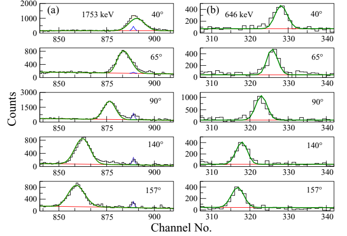
FIG. 4. Representative fits to the Doppler shapes observed for (a) 1753-keV and (b) 646-keV transitions belonging to Band-I and Band-II, respectively, of ^{29}\text{Al} . The contaminant stopped peak, as indicated in panel (a), belongs to ^{26}\text{Mg} .
