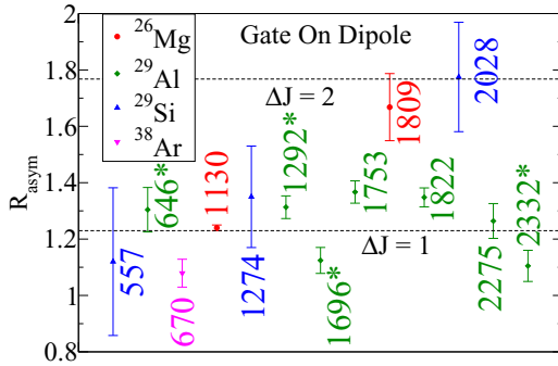
FIG. 3. The R_{\text{asym}} values for the transitions of present interest in ^{29}\text{Al} . The fitted values for the transitions (with known multiplicities) of a few other residual nuclei, populated in the same reaction, have also been depicted for comparison. The \Delta J = 1 and \Delta J = 2 lines have been drawn to guide the eye. The transitions belonging to Band-II of ^{29}\text{Al} have been marked with *.
