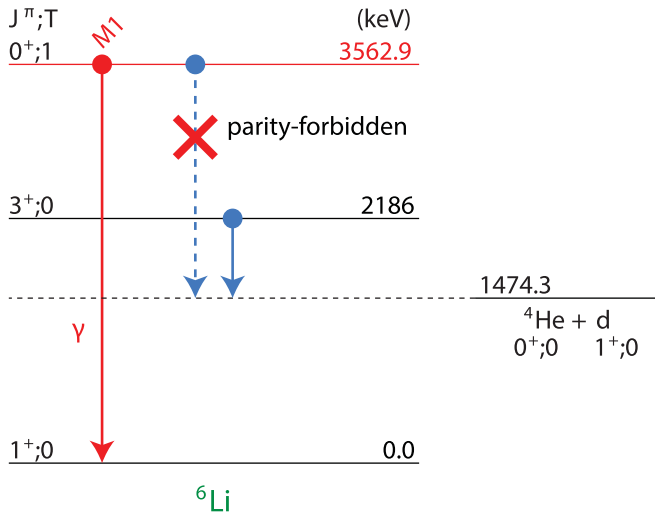
FIG. 1. A simplified level diagram of {}^6\text{Li} based on Ref. [35]. The \alpha decay of the J^\pi = 0^+, T = 1 state at E_x = 3.56 \text{ MeV} is isospin and parity forbidden, and this state decays to the ground state via \gamma emission [36,37].
