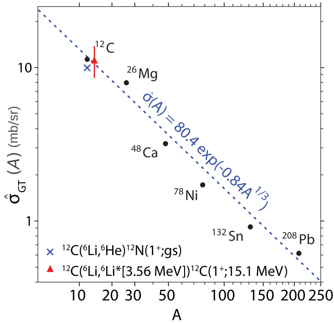
FIG. 5. GT unit cross section for the ( {}^6\text{Li} , {}^6\text{Li}^*[3.56 \text{ MeV}] ) reaction at 100 MeV/u as a function of target mass number. The red marker is the extracted unit cross section for the {}^{12}\text{C}({}^6\text{Li}, {}^6\text{Li}^*[3.56 \text{ MeV}]){}^{12}\text{C}(15.1 \text{ MeV}) reaction from the present paper. The blue marker refers to the unit cross section from Ref. [50] for the analog transition measured in a {}^{12}\text{C}({}^6\text{Li}, {}^6\text{He}) experiment at 100 MeV/u. The black markers refer to calculated unit cross sections in DWBA, and the blue dashed line is a fit to these unit cross sections. For details, see the text.
