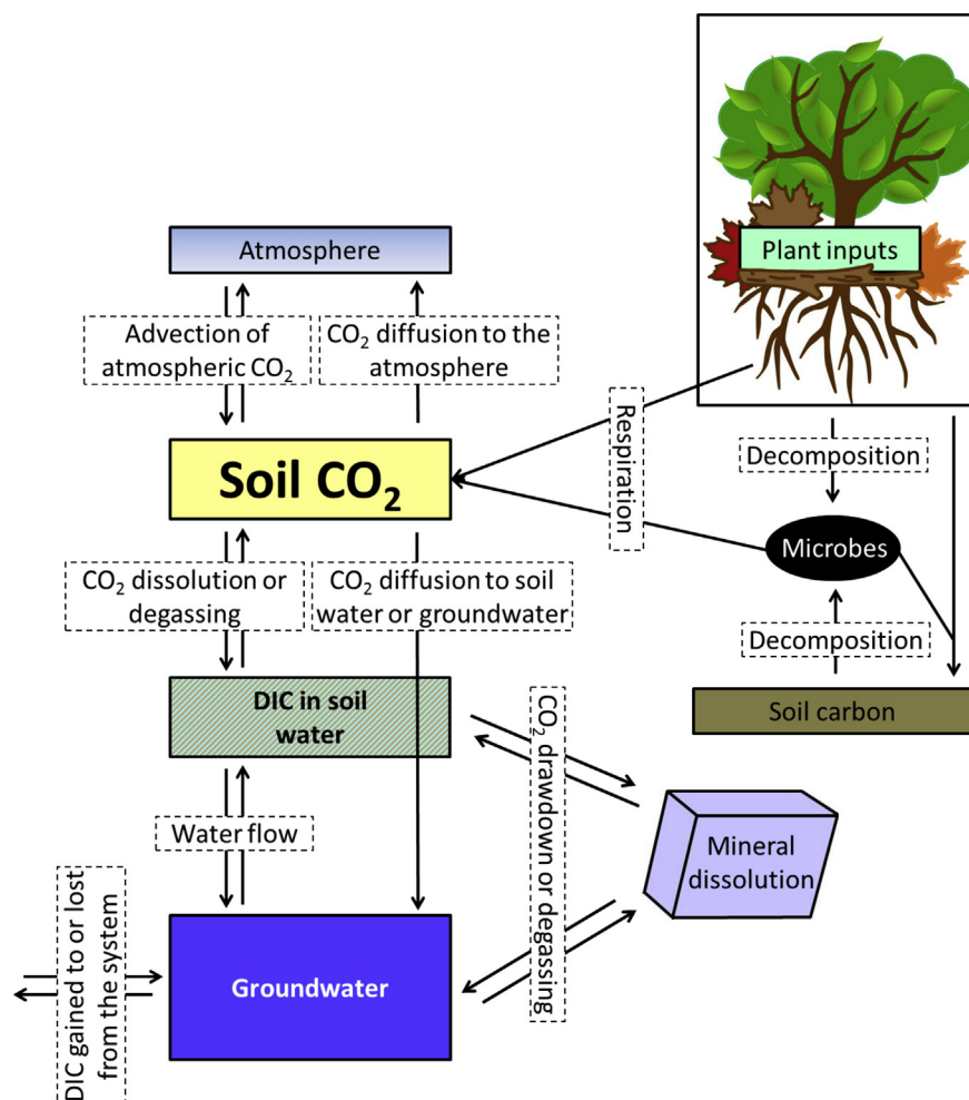
Fig. 1. Soil atmosphere pCO 2 reflects the balance of i) production of CO 2 by belowground cellular respiration, ii) diffusion of CO 2 out of the soil upward to the atmosphere or downward to soil water or groundwater, iii) CO 2 drawdown from or CO 2 degassing to porefluids during mineral dissolution (this process depends on what mineral(s) dissolve), iv) advection of dissolved inorganic C (DIC)-containing fluid into or out of the system, and v) advection of atmospheric CO 2 into air-filled soil pore spaces.
