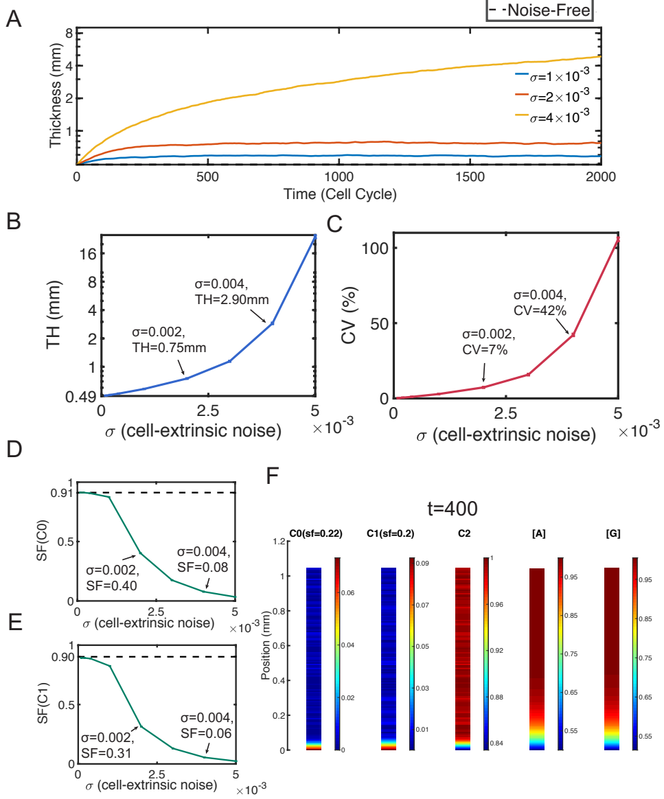
Figure 4. Simulations with only cell-extrinsic noise. Dash lines represent the corresponding quantities at homeostasis. A. Layer thickness in three simulations with \sigma = 1 \times 10^{-3} , 2 \times 10^{-3} and 4 \times 10^{-3} . B. The mean TH . The error bars show the standard deviation. C. The mean CV . The error bars show the standard deviation of CV . The mean SF of D. stem cells and E. TA cells. The error bars show the standard deviation. F. Distribution of cells and morphogens in a specific simulation with \sigma = 3 \times 10^{-3} at time t = 400 . In (B-E) , all statistical quantities are captured based on 20 simulations, and the standard deviations (error bars) are negligible compared to the means.
