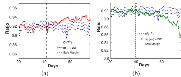
Fig. 16. Incremental Evolving Attack: (a) Additive (b) Camouflage
