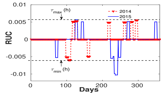
Fig. 8. Standard Limits of RUC with \kappa = 2s_r
