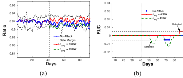
Fig. 22. Worst Case \delta_{avg} \sim k_{low} : (a) Ratio (b) RUC
