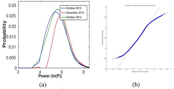
Fig. 1. Texas Data (a) p^{mix} for different months (b) The Q-Q Plot
