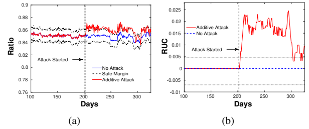
Fig. 18. Irish DataSet: Additive: (a) Ratio (b) RUC
