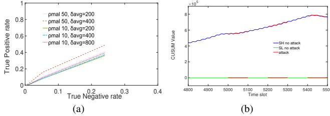
Fig. 23. Comparison: (a) EWMA (b) CUSUM
