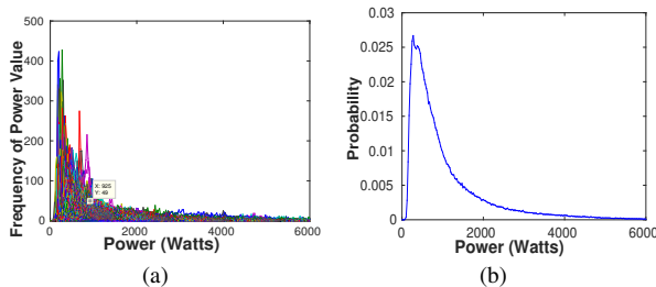
Fig. 3. Power Consumption (Texas, US): (a) 200 houses (b) Mixture P^{mix}
