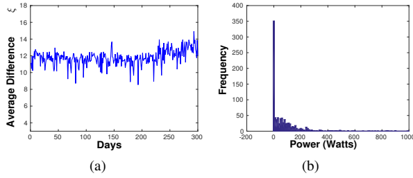
Fig. 10. Irish Dataset: (a) Average Difference \xi(T) (b) a_{min} values
