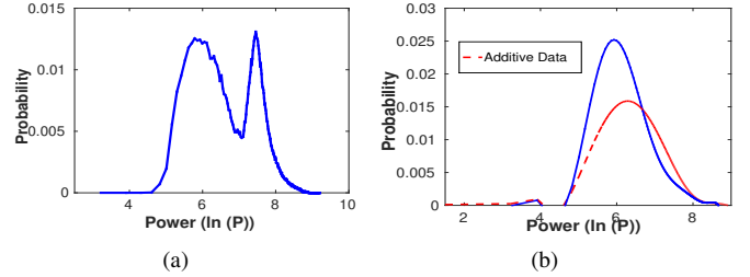
Fig. 2. Attack Distributions (a) Obvious Attack (b) Smarter Attack
