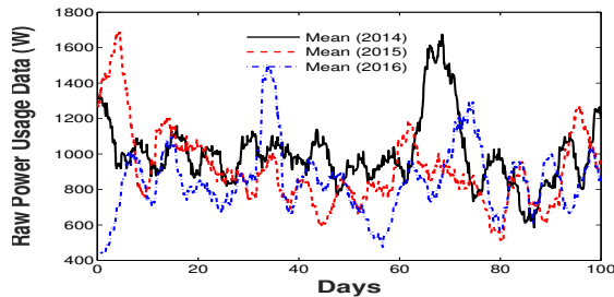
Fig. 1. Instability of mean power consumption
