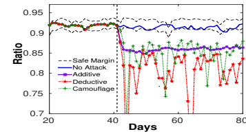
Fig. 19. High Attack Strengths: \Delta_{avg} = 800
