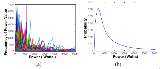
Fig. 4. Power Consumption (Ireland): (a) 5000 houses (b) Mixture P^{mix}
