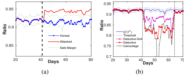
Fig. 15. Low attack strength (a) Additive (b) All Mixed
