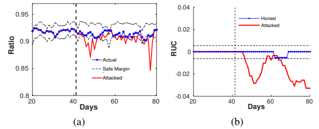
Fig. 9. Ultra Low Camouflage (a) Ratio (b) RUC
