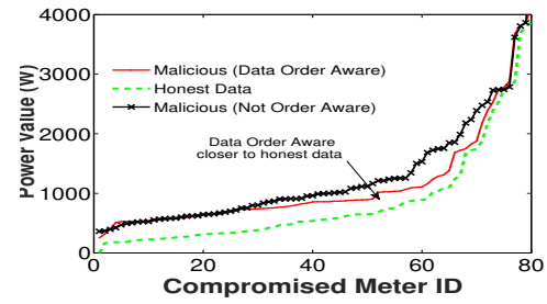
Fig. 2. Illustration: Benefit of Data Order Awareness
