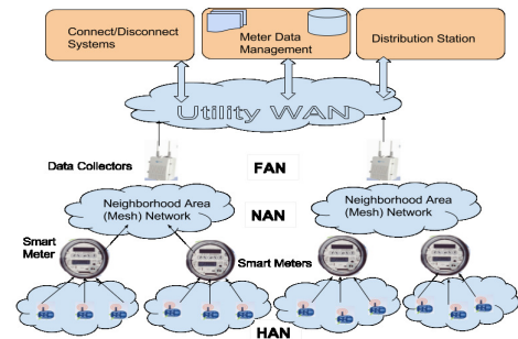
Fig. 5. AMI: Generic System View
