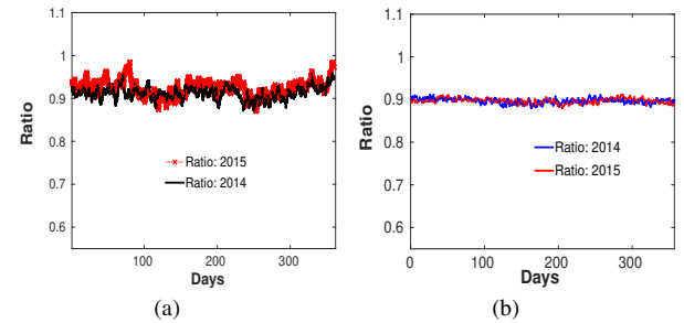
Fig. 6. Legitimate HM/AM Ratio: (a) 200 meters (b) 800 meters
