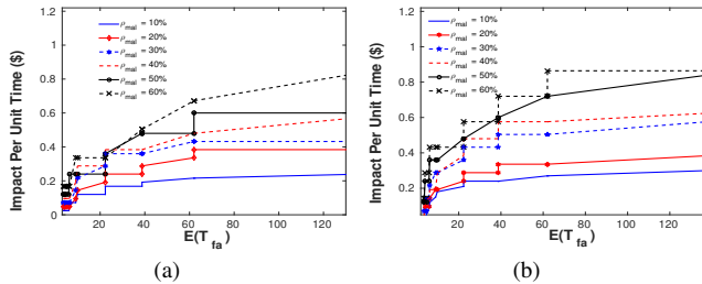
Fig. 20. Limiting Impact of Persistent Attacks: (a) Deductive (b) Additive
