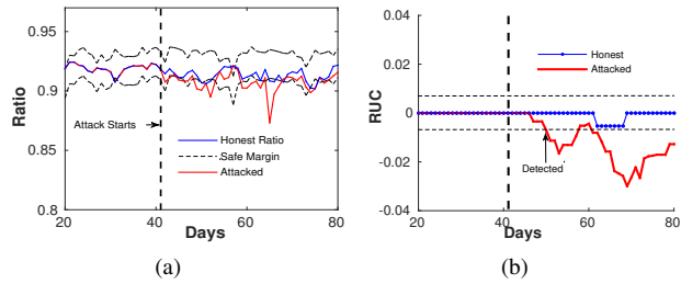
Fig. 13. Ultra Low Deductive (a) Ratio (b) RUC
