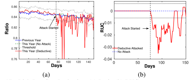
Fig. 17. Irish DataSet: Deductive: (a) Ratio (b) RUC
