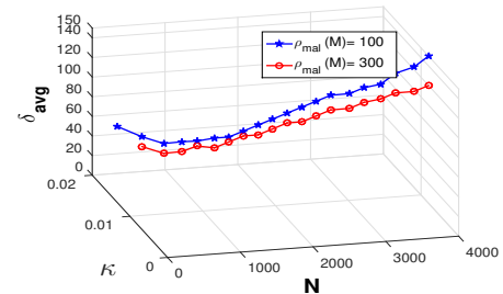
Fig. 21. Scalability and Sensitivity Performance: Irish Dataset
