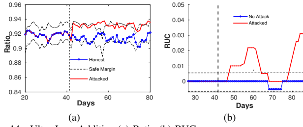
Fig. 14. Ultra Low Additive (a) Ratio (b) RUC
