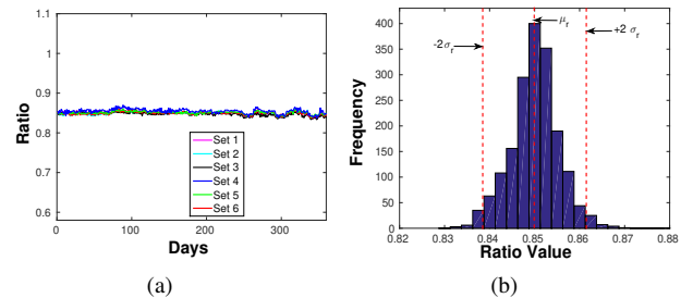
Fig. 7. Irish Data (5000 meters; 6 regions): (a) Ratios (b) Ratio Distribution
