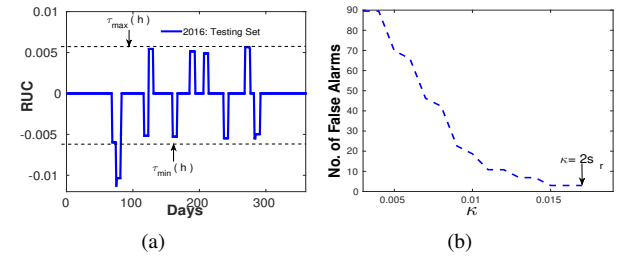
Fig. 12. False Alarm Performance(a) All \kappa (b) N = 800 with \kappa = 2s_r
