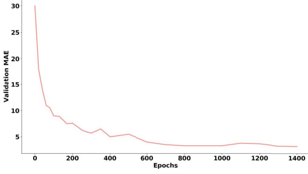
Fig. 3: MAE vs. Epoch curve during training of travel time prediction model.
