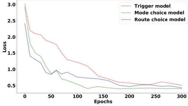
Fig. 4: Loss vs. Epoch curve during training of agent models.
