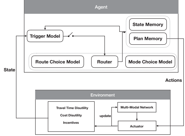
Fig. 1: Mobilitycs-Gym architecture
