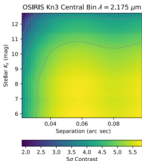
Fig. 18 The colorscale shows the 5\sigma single companion contrast for OSIRIS kernel phase observations as a function of target star apparent magnitude and angular separation. The gray-dotted lines show 1 magnitude increments in companion contrast.
