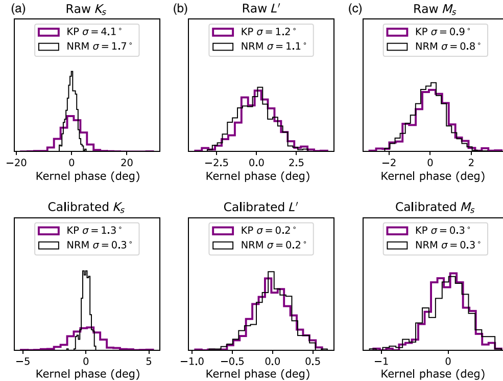
Fig. 24 Histograms of raw (top) and calibrated (bottom) kernel phases for (a) K_s , (b) L' , and (c) M_s band NIRC2 observations for a bright (sixth apparent magnitude) target star. Thick purple lines show filled-aperture kernel phases, while thin black lines show NRM kernel phases.
