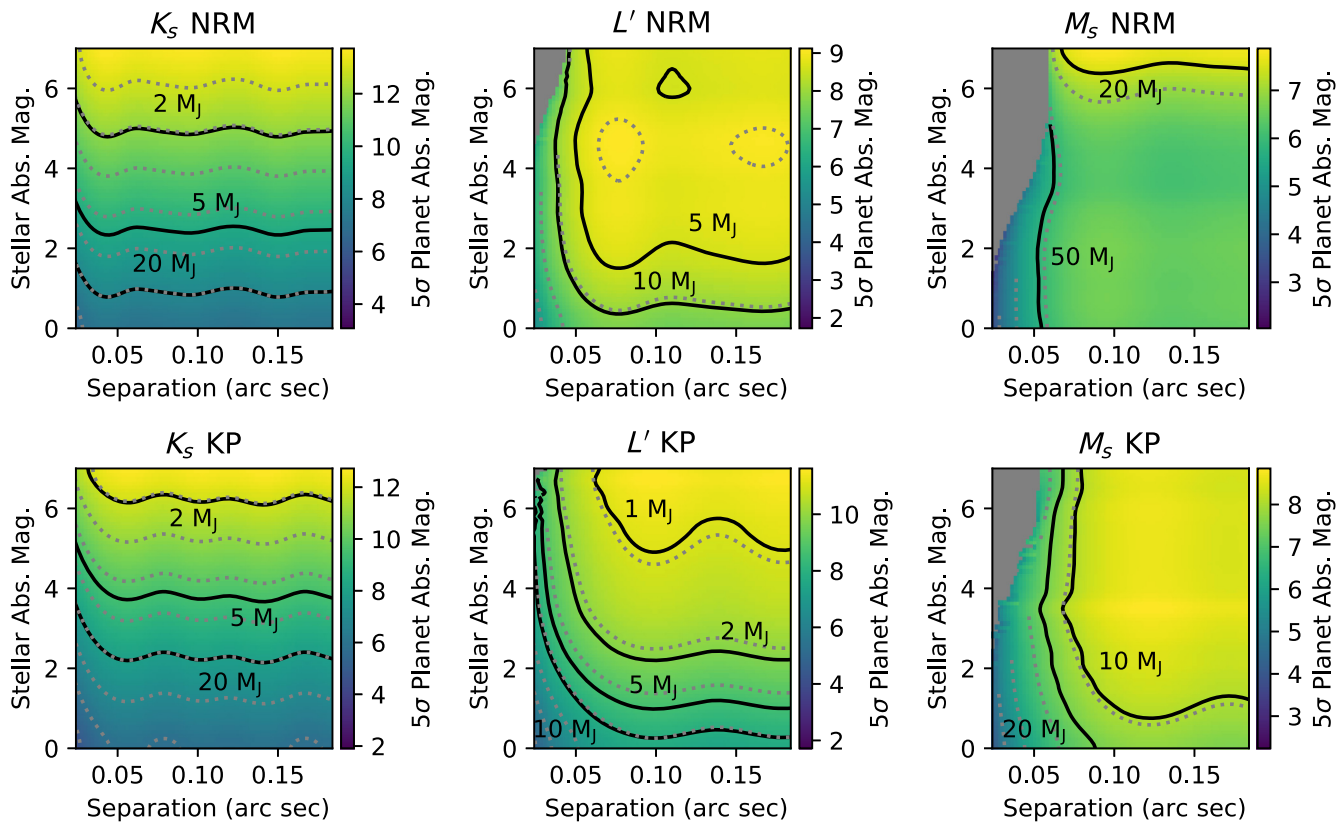
Fig. 12 Five \sigma planet mass limits using 1 Myr DUSTY models (solid lines) for all NIRC2 bandpasses and both techniques. The color scale shows the 5\sigma absolute companion magnitude, calculated using the contrasts shown in Fig. 11 and by translating the stellar apparent magnitudes to absolute magnitudes at 140 pc. Gray-shaded regions are regions of the parameter space where no companion model was significant at the 5\sigma level, compared to the null (single point source) model. The gray-dotted lines show 1 magnitude increments in absolute companion magnitude. The changing noise regimes (OPD error dominated to random error dominated) in the L' and M_s NRM simulations cause the achievable contrast to fall off nonuniformly as the target brightness changes (see Fig. 11, upper center and upper right panels). This causes local regions in the L' and M_s stellar magnitude—separation parameter space to be better suited for detecting lower planet masses (see upper center and upper right panels here, colorscale and contours).
