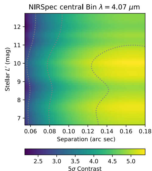
Fig. 21 The colorscale shows the 5\sigma single companion contrast for NIRSpect kernel phase observations as a function of target star apparent magnitude and angular separation. The gray-dotted lines show 1 magnitude increments in companion contrast.
