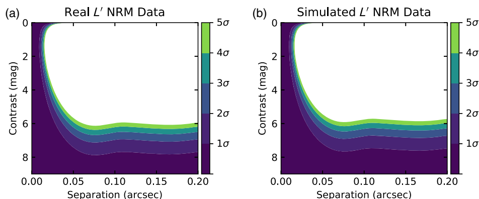
Fig. 9 Contrast curves for a single target observation made from (a) real L' NIRC2 NRM observations and (b) simulated observations. The contrast curves are nearly identical, with 5\sigma contrast of >5.5 magnitudes.
