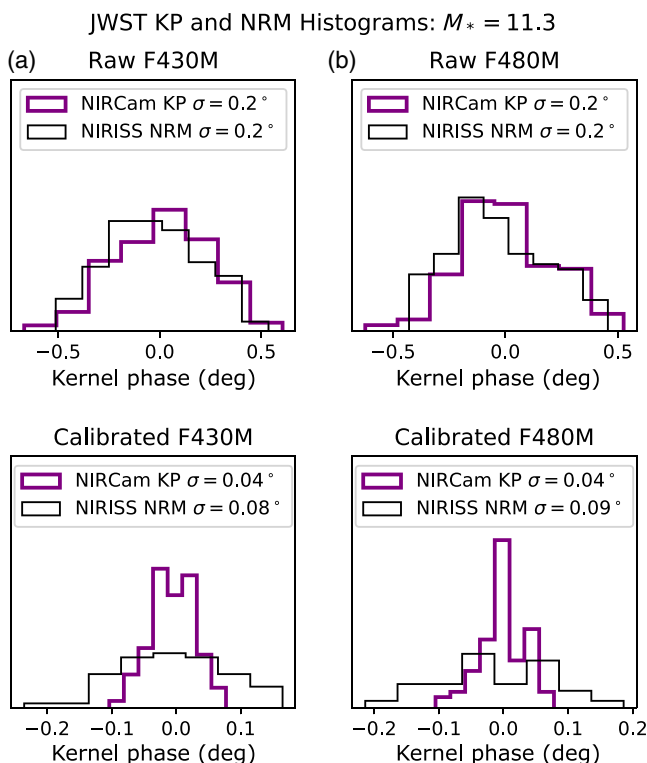
Fig. 27 Histograms of raw (top) and calibrated (bottom) kernel phases for (a) F430M and (b) F480M band observations for a faint (11th apparent magnitude) target star. Thick purple lines show NIRCam filled-aperture kernel phases, while thin black lines show NIRISS NRM kernel phases.
