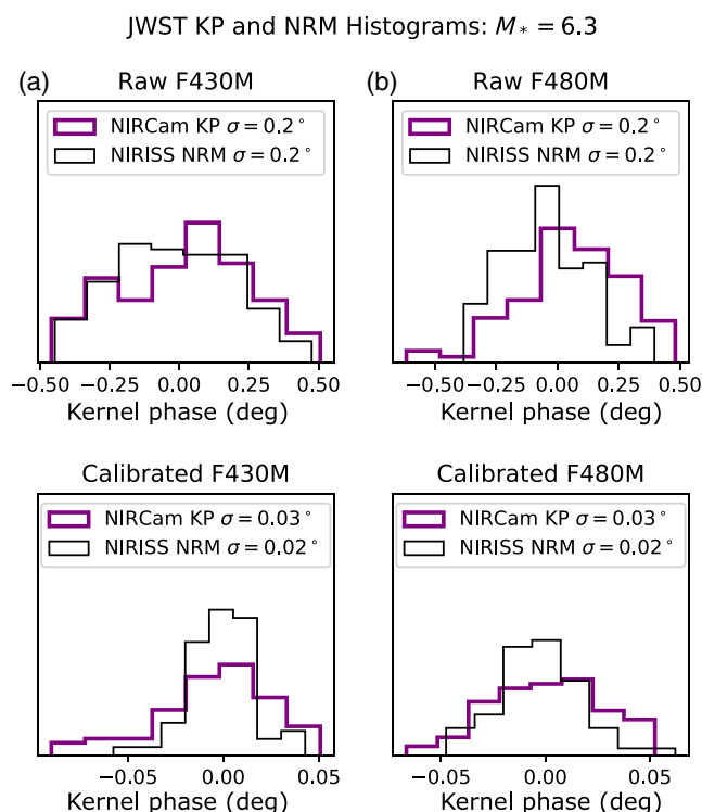
Fig. 26 Histograms of raw (top) and calibrated (bottom) kernel phases for (a) F430M and (b) F480M band observations for a bright (sixth apparent magnitude) target star. Thick purple lines show NIRCam filled-aperture kernel phases, while thin black lines show NIRISS NRM kernel phases.
