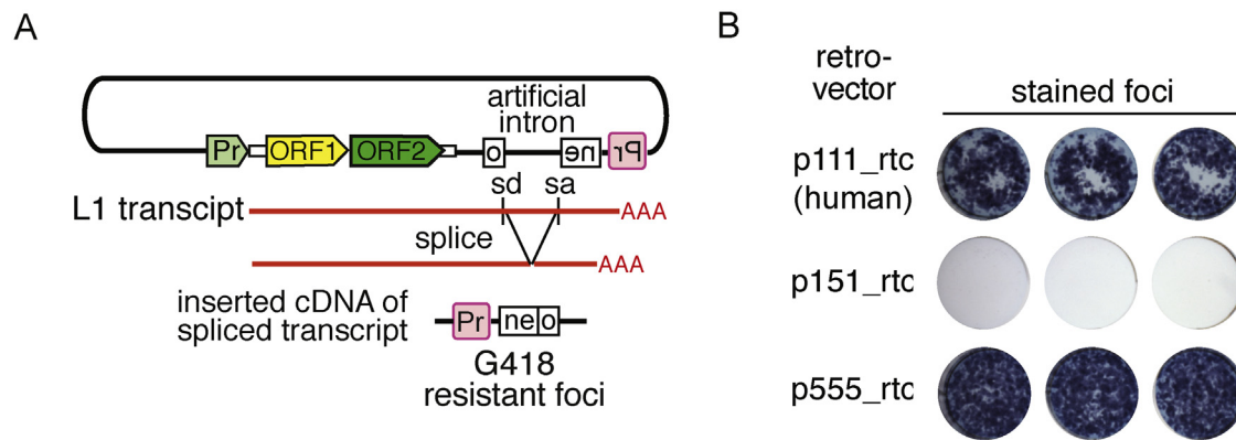
Fig. 7. Retrotransposition assay. A) Organization of an L1 vector in a typical retrotransposition assay. The L1 vector contains an antisense copy of the neo gene disrupted by an intron in the sense orientation. sd and sa are the splice donor and splice acceptor sites, respectively. The intron of the transcribed L1 vector will be spliced and contain the antisense copy of the neo gene. Retrotransposition competent elements will support subsequent cDNA synthesis of this transcript at a DNA target site and ultimately the insertion of an active copy of the neo gene, which when expressed from its promoter (Pr, in red) generates colonies of G418 resistant cells or foci. B) An example of stained foci generated from the retrotransposition assay described in (A) [43]. p111_rtc, p151_rtc and p555_rtc are the L1 vectors containing the modern human, mosaic and the resuscitated primate ORF1 sequences (see inset of Fig. 6B), respectively.
