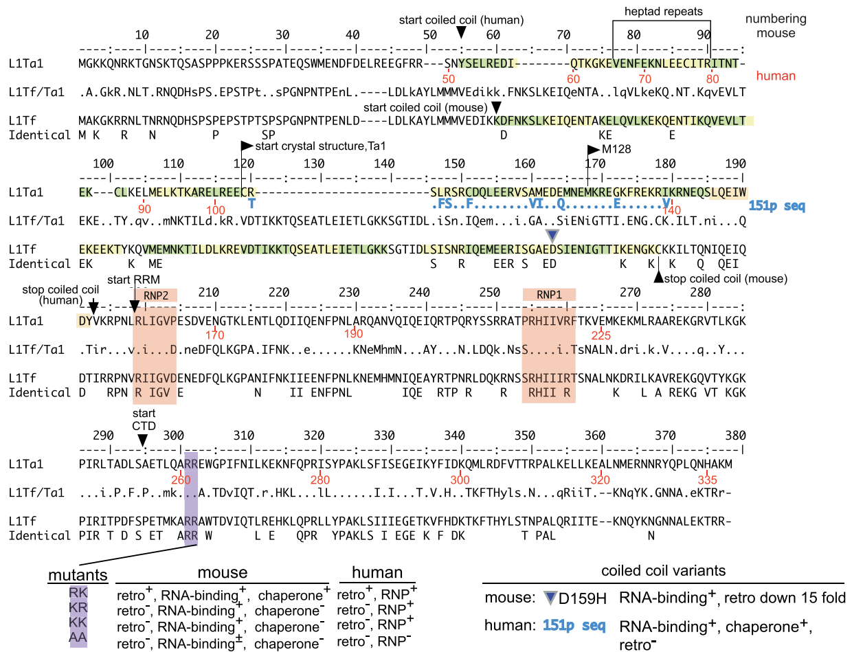
Fig. 2. Alignment of mouse and human ORF1p sequences. Consensus sequences of the mouse L1Tf family [13] and the human Ta1 subfamily of the currently active L1Pa1 [15] family were aligned. The middle L1Tf/Ta1 sequences shows the comparison between the aligned elements. A dot indicates identity, dashes indicate gaps, and lower case indicates conservative amino acid differences. The bottom entry (Identical) shows the 100% identical positions. The numbers in black refer to the L1Tf, and those in red, the L1Ta1 sequence. The beginning and end of the coiled coil domain, and the starts of the RNA recognition motif (RRM) and C-terminal domain (CTD) are indicated. The coordinates of the RRM and CTD were taken from references [36,47]. The alignment is also annotated with the following information: The beginning of truncated M128 [44], which is largely a monomer at \geq 20^\circ\text{C} ; the location of a natural variant in the mouse coiled coil domain (D159H, using the L1Tf numbering with an offset of plus 4 in the mouse alignment only to account for the 4 position gap introduced into the alignment of L1Tf between positions 40 and 45) [41,26,38,46] paired mutations in two adjacent highly conserved arginine residues of the CTD, in human ([26,29]) and in mouse [42]. Heptad repeats are highlighted in green and yellow. RNP1 and RNP2 sequences are highlighted in light brown [36]. Regarding the “phenotype” of these mutations: retro means retrotransposition as measured in a cell culture based retrotransposition assay [26]; RNP means the presence of ORF1p in RNP particles isolated from in vivo assays; RNA binding means as performed with purified ORF1p protein in vitro ; chaperone means chaperone activity (as described in [42]).
