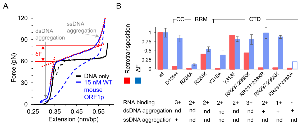
Fig. 5. Single molecule DNA stretching results from mouse ORF1p mutational analyses [41,42,59]. Solid and dashed blue lines are the stretch and return curves of dsDNA in the presence of 15 nM wild type mouse ORF1p. \Delta F is the relative increase in the helix-coil transition width due to bound protein, where \Delta F = \delta F - \delta F_0 . Here, \delta F_0 (~4 pN) and \delta F are the helix-coil transition widths in the absence and presence of protein, respectively. \delta F (shown as the force difference between the solid red lines) is determined by the intersection of the dashed red lines on the figure, which represent ds- and ss- DNA regimes of the ORF1p-DNA complex. Thus, \Delta F is a measure of the relative increase in force (due to bound protein) required in the cooperative conversion of ds- to ss- DNA, which was shown to be positively correlated with the nucleic acid chaperone capabilities of the bound protein as described in the text. B) \Delta F at 15 or 20 nM protein concentration, as measured in single molecule DNA stretching assays (blue), and retrotransposition activity in cultured in vivo assays (red) for ORF1p mutants, presented after normalizing with the corresponding values for the wild type protein. The transition width for the RR297:298AA mutant at these concentrations was not reported due to its lower binding affinity. However, it was shown to saturate at a 5-fold higher concentration than what was used for wild type protein. The empty bar is to denote that the transition width is likely much smaller at these concentrations in comparison with the wild type protein. Extensive aggregation of single- or double- stranded DNA in comparison with the wildtype protein, are denoted with a plus sign. While aggregation is important to facilitate DNA interactions and can increase chaperone activity, extensive aggregate formation can also slow down DNA interaction kinetics, which may in turn inhibit chaperone activity [79]. The ability to bind RNA as observed in the bulk solution assays is also reported. The plus sign denotes comparable binding affinity as wild type and these mutants are ranked according to their relative binding affinities, with (-) the lowest and (3+) the highest affinity. 'nd' represents 'not determined'.
