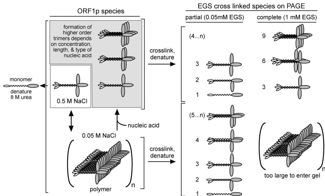
Fig. 3. ORF1p polymerization. Schematic representation of possible ORF1p species and their cross-linked products as observed in Callahan et al. [44]. The numbers to the left of the cartoons of the cross-linked species indicate their monomer content. 4..n and 5..n indicate higher orders of multimers beyond 3 or 4, respectively. Higher orders of ORF1p multimers of trimers were observed in crosslinking experiments with 1 mM EGS, in the presence of oligonucleotides at 0.05 M NaCl.
