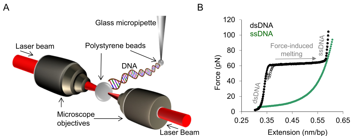
Fig. 4. Single molecule DNA stretching. A) Schematic depiction of an optical tweezers system. A single molecule of \lambda DNA (48.5 kbp) is attached by its biotinylated ends to streptavidin-coated polystyrene beads. One bead is immobilized by a glass micropipette attached to a flow cell while the other is held in an optical trap. The optical trap is created by converging two counter-propagating laser beams to overlap in space using microscope objectives. By moving the glass micropipette attached to the flow cell, the tethered DNA molecule is stretched, and the force exerted on the DNA is measured as a function of extension in the presence and absence of protein. B) Solid and empty black circles (also the solid and dashed black lines in Figs. 5A and 6A) represent the stretch and return curves of a bare dsDNA molecule. The green circles represent the force-extension curve of an ssDNA molecule. The distinct regimes of the dsDNA force-extension profile are denoted in grey text. At forces \ll \sim 60 pN the DNA molecule is primarily double-stranded. The plateau at \sim 60 pN represents a sharp overstretching transition, where very little additional force causes the DNA molecule to stretch to almost twice its contour length. This is due to force-induced melting of the DNA molecule and this transition is referred to as the helix-coil transition [73]. The force range over which this transition occurs is defined as the helix-coil transition width (or transition width). In the salt conditions used in these studies, the stretched dsDNA molecule is mostly single-stranded at forces higher than the helix-coil transition. The stretch and return cycles of the bare DNA molecule are almost reversible and immediate re-annealing of the duplex is observed when the stretched DNA molecule is returned to zero-force (empty black circles).
