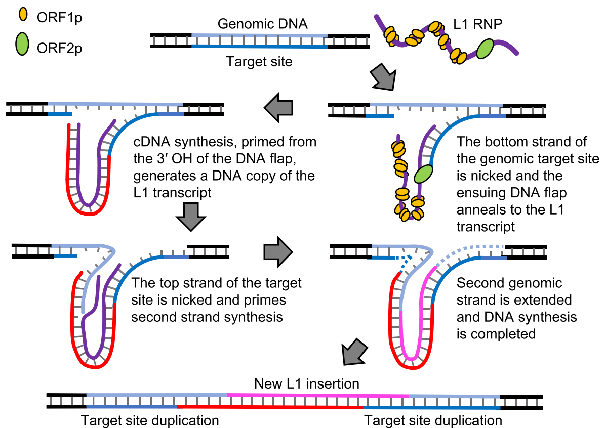
Fig. 1. A) L1 domain structure. The domain organization of a typical full-length human L1 element. Approximate positions (not to scale) of the 5' untranslated region (5' UTR), ORF1, ORF2 (which includes endonuclease (EN) and reverse transcriptase (RT)), 3' UTR, and the poly A tail are noted. B) Domain structure and trimeric depiction of ORF1p. The amino acid positions of the N-terminal domain (NTD), coiled coil domain (CC); RNA recognition motif (RRM) and C-terminal domain (CTD) for mouse [13,40,47,55] and human [36,44,46] ORF1p are denoted in red and blue text, respectively. C) Schematic of the proposed steps in TPRT [3,31,32]. Target site of the genomic DNA is depicted in blue shades and L1 RNA in purple. The first DNA strand at the target site is cleaved by ORF2p EN. The L1 RNA is annealed to the cleaved site and reverse transcribed by ORF2p RT to synthesize the first L1 cDNA (red). The second genomic target site strand is cleaved, and it primes the L1 cDNA to synthesize the second L1 DNA strand (magenta). Subsequent DNA synthesis required for completion is denoted in dashed lines. Consequently, target site duplications (TSD) are produced at the flanks of the newly synthesized L1 element. ORF1p may mediate strand exchange reactions required to anneal the primers and/or facilitate nucleic acid arrangements during reverse transcription.
