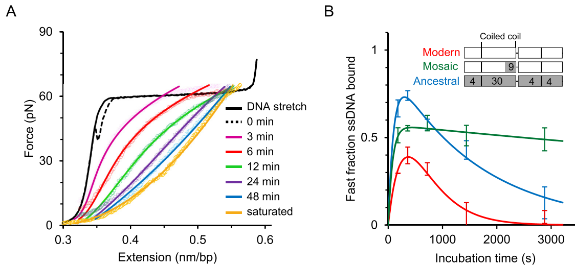
Fig. 6. Single molecule studies of human ORF1p [43]. A) In contrast to the studies described in Fig. 5, here, the DNA molecule is overstretched above the helix-coil transition up to the ssDNA regime before incubating it with the protein, in order to minimize dsDNA binding effects and exclusively investigate ssDNA-ORF1p binding kinetics. Solid and dashed line represent the stretch-return cycle of a bare dsDNA, with the return curve also referred to as 0 min incubation. The colored empty circles are the return curves of a DNA molecule after incubating with 2 nM protein at ~70 pN for different time periods. The gold curve listed as saturated represents the maximum shift in extension towards ssDNA, obtained at long incubation times and greater than 15 nM protein concentration. The ssDNA-bound protein during the incubation prevents reannealing and thereby shift the relaxation curve after protein incubation towards the ssDNA curve (see green circles, Fig. 4B), allowing one to quantitatively probe the ssDNA fraction bound as a function of time. The solid lines represent the fitted curves as described elsewhere [43]. ORF1p rapidly binds ssDNA. However, it transforms relatively slowly into stable oligomers. Less stable proteins (presumably un-transformed trimers) dissociate during the return cycle and the ssDNA fraction bound by such proteins is defined as the fast fraction in this study. The fast fraction decreases with incubation time as they transform into more stable oligomers on ssDNA. B) Fast fraction as a function of time for modern human (111 p, from L1Pa1 family), its resuscitated ancestral primate (555 p, from L1Pa5 family) and a mosaic ORF1p (151 p) in which 9 residues in the coiled coil are replaced with the corresponding ancestral residues, as shown in the inset (also see Fig. 2 where these residues are indicated in teal). Domain boundaries in the inset correspond to Fig. 1B and white and grey shades represent the amino acid residues of the modern and ancestral ORF1p, respectively. The number of amino acid substitutions relative to the modern ORF1p is denoted in the relevant domains in the other two ORF1p variants. The measured fast fraction is modeled as a sum of increasing and decreasing exponential functions (solid lines) and red, blue and green represent modern, ancestral, and mosaic proteins, respectively. The fast fraction rapidly saturates for all three variants, indicating rapid protein binding to ssDNA. However, this fraction decreases with increasing incubation time as the proteins form more stable oligomers. Therefore, the rate at which the fast fraction decreases is proportional to the rate of stable oligomerization of protein on ssDNA. The retrotransposition-incompetent mosaic ORF1p was at least 10-fold slower in forming stable oligomers in comparison with the active human and primate protein variants.
