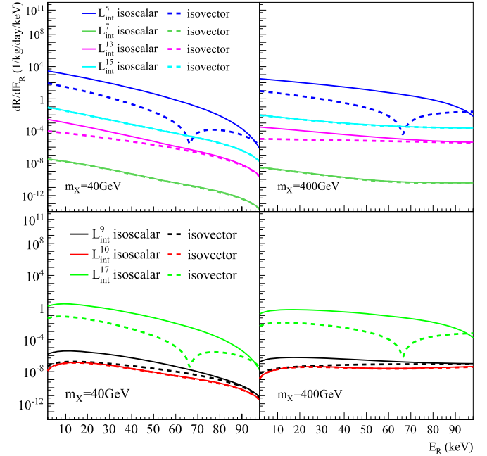
Fig. 1. Recoil energy spectra for the scattering of spin- \frac{1}{2} WIMPs on xenon nuclei, for WIMP masses of 40 \text{GeV}/c^2 and 400 \text{GeV}/c^2 , and unit isoscalar ( d_i^0 = 1, d_i^1 = 0 ) and isovector ( d_i^0 = 0, d_i^1 = 1 ) coupling. Top panel: dimension-four V-A interactions. Bottom panel: higher dimension magnetic and electric dipole interactions.
