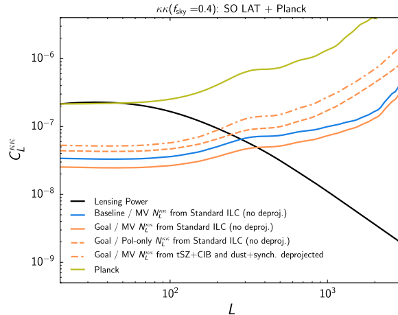
Figure 6. \Lambda CDM CMB lensing power spectrum (black) compared to SO LAT lensing noise curves, N_L^{KK} , reconstructed assuming a polarization only (Pol-only) or minimum variance (MV) combination of estimators in the case of standard ILC for both CMB temperature and polarization cleaning (solid and dashed curves), and tSZ and fiducial CIB SED deprojection for CMB temperature cleaning and fiducial polarized dust and synchrotron SED deprojection for CMB polarization cleaning (dot-dashed curve). SO baseline and goal scenarios are shown in blue and orange, respectively, and compared to the Planck lensing noise ([288], yellow). SO will be able to map lensing modes with S/N > 1 to L > 200 .
