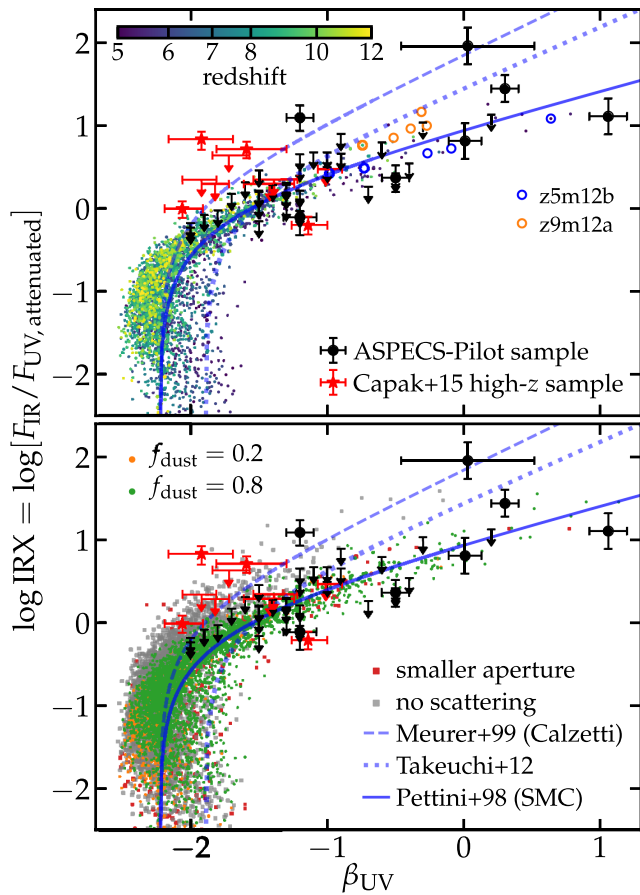
Figure 5. Top: The IRX– \beta_{UV} relation for our simulations (using f_{\text{dust}} = 0.4 ). Each point represents a galaxy snapshot along a random line of sight, colour-coded by redshift. Galaxies at higher redshifts tend to move slightly towards bluer \beta_{UV} at fixed IRX due to their younger stellar populations. Points with errorbars show the observational data sets for high-redshift galaxies compiled in Casey et al. (2018b), consisting of two different samples). The lines show the empirical relations from the literature. The simulated sample forms a tight IRX– \beta_{UV} relation broadly agrees with observations and the SMC IRX– \beta_{UV} relation expected from a simple dust screen model. Our results suggest that patchy, complex dust distribution and non-trivial effect of dust scattering as shown in our simulations do not drive significant scatter in the IRX– \beta_{UV} relation. Bottom: The IRX– \beta_{UV} relation for different normalizations of the extinction curve (represented by varying f_{\text{dust}} ; the colour points). The grey squares show the results if dust scattering is ignored, which should be understood as changing the attenuation law. These results confirm that the IRX– \beta_{UV} relation is determined by the shape of the extinction curve but independent from its normalization. The red squares show the results if the IR and UV fluxes are measured in a smaller aperture ( R_{\text{max}}/3 instead of R_{\text{vir}} ), which has little effect on the results.
