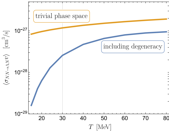
FIG. 2. (Left) The value of \langle\sigma_{NN\rightarrow \Lambda N}v\rangle with and without phase-space degeneracy effects. (Right) The coupling g_{\Lambda S}^2 from wave function overlap, as a function of r_S for two different values of r_\Lambda , as in Eq. (B1). In the gray region, r_S violates Eq. (9) for x = 0.1 .
