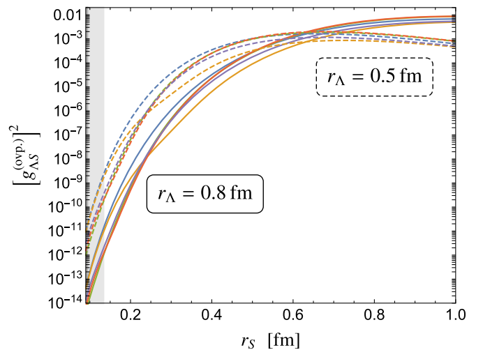
FIG. 2. (Left) The value of \langle\sigma_{NN\rightarrow \Lambda N}v\rangle with and without phase-space degeneracy effects. (Right) The coupling g_{\Lambda S}^2 from wave function overlap, as a function of r_S for two different values of r_\Lambda , as in Eq. (B1). In the gray region, r_S violates Eq. (9) for x = 0.1 .
