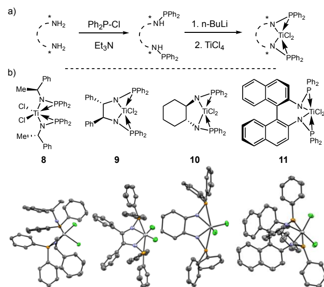
Figure 3. a) Synthesis route for chiral titanium phosphinoamide ligands. b) Structure and X-ray structure of titanium ligands synthesized.
