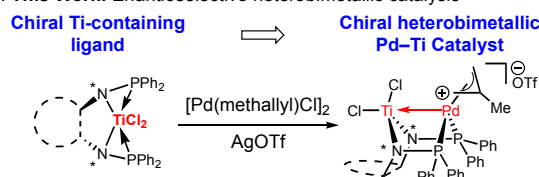
Figure 1. Examples of bimetallic catalysts and the chiral heterobimetallic catalyst used in this work.
