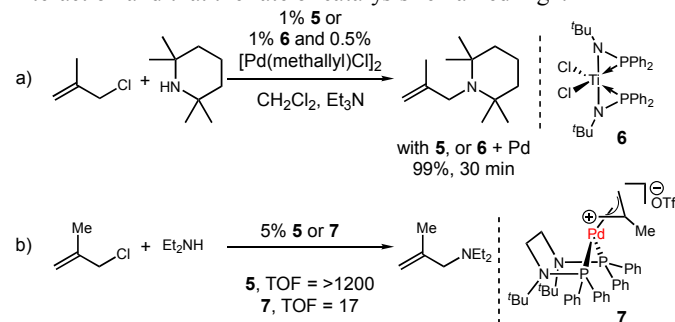
Figure 2. Allylic amination with Ti-Pd catalysts.
