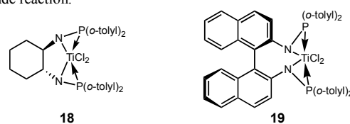
Figure 5. o -Tolyl-substituted titanium ligands.
