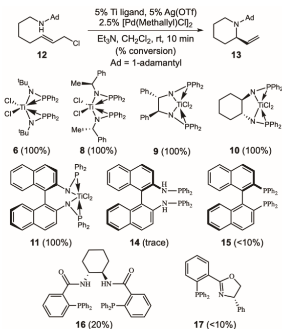
Figure 4. Ligand reactivity study. Numbers in parentheses represent reaction conversions by comparing the ratio of product to remaining starting material.
