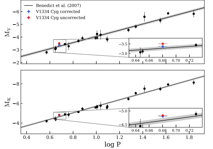
Figure 5. Period–Luminosity relations constructed from direct parallax measurements. This includes our measured distance and those from Casertano et al. (2016), Riess et al. (2018), and Benedict et al. (2007, 2002). We also included the distance estimated from light echoes by Kervella et al. (2014). The blue and red dots represent the location of V1334 Cyg for companion-flux corrected and uncorrected magnitude, respectively. Uncertainty on the fundamentalized period is also shown. The relation derived by Benedict et al. (2007) is also plotted, with the rms of the residuals in the shaded area.
