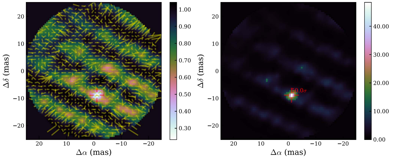
Figure 1. \chi^2 map of the local minima (left) and detection level map (right) of V1334 Cyg for the 2012 July observations. The yellow lines represent the convergence from the starting points to the final fitted position, as explained in Gallenne et al. (2015). The maps were re-interpolated in a regular grid for clarity. The axis limits were chosen according to the location of the companion.
