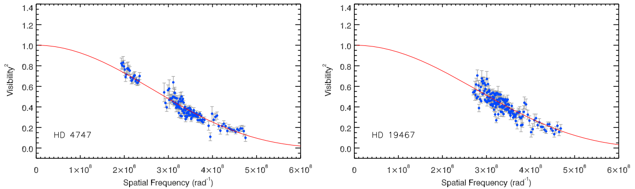
Figure 1. Calibrated interferometric V^2 values (points) and the R -band, limb-darkened fits to those measurements (line) for HD 4747 (left) and HD 19467 (right). The units of the x -axis correspond to the baseline length in units of operational wavelength. For more details, see Section 2.
