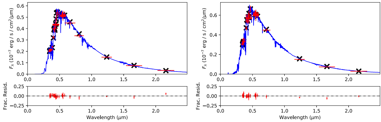
Figure 2. SED fits for HD 4747 A (left) and HD 19467 A (right). Pickles (1998) spectral templates (blue lines; G8V for HD 4747 A, G2V for HD 19467 A) are scaled to the literature photometry (red crosses). Black crosses show the flux value of the spectral template integrated over the filter transmission profile. The lower panels display residuals between literature photometry and the spectral template. See Section 3 for more details.
