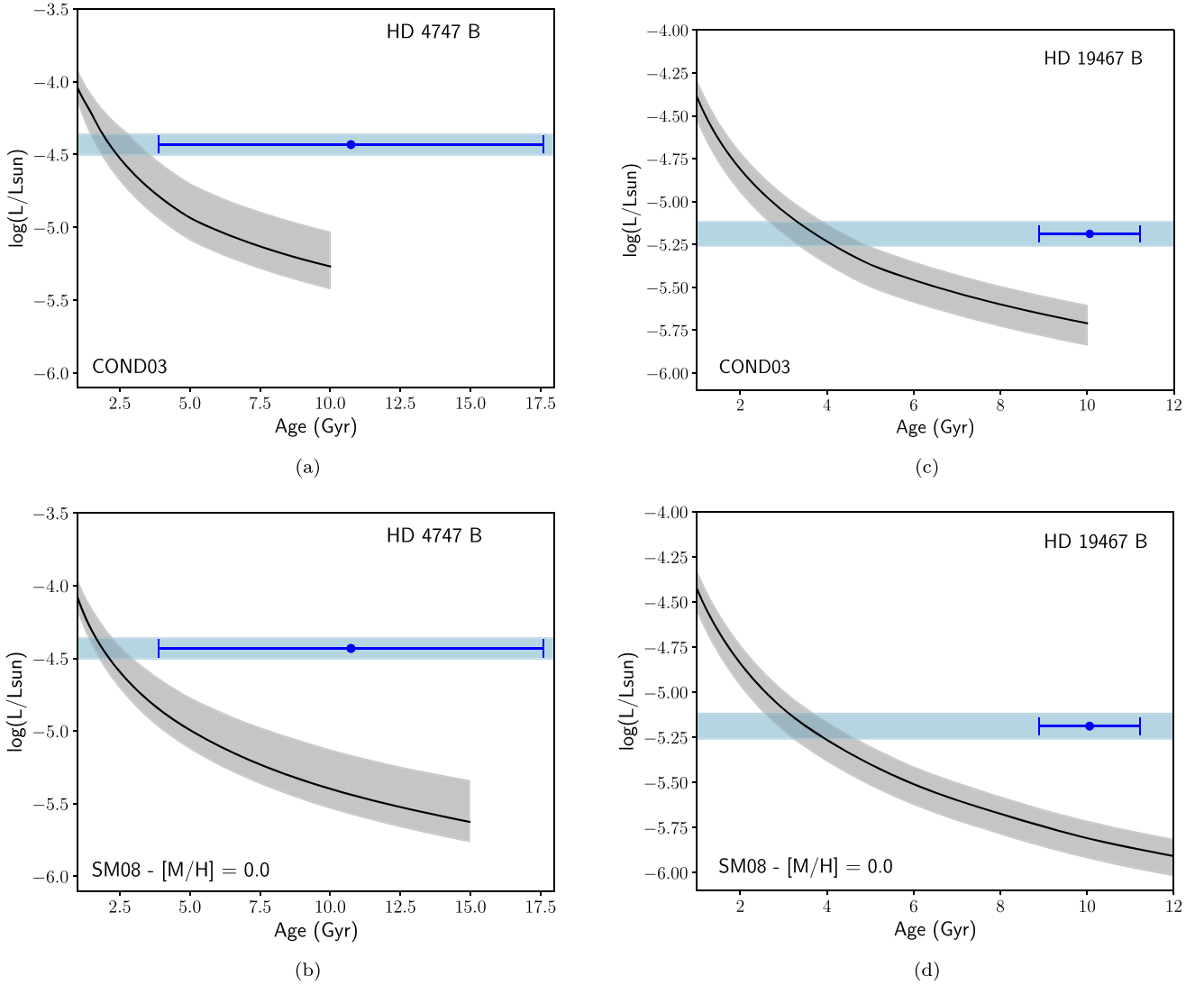
Figure 4. Luminosity vs. age comparison of the COND03 and SM08 substellar evolutionary models (black curves) to the observed data (blue dots) for HD 4747 B (a) and (b) and HD 19467 B (c) and (d). The light blue bars correspond to the uncertainty in the bolometric luminosities for the brown dwarfs. Although the models do not extend past 10 Gyr (COND03) and 15 Gyr (SM08), it is clear that they under-predict the bolometric luminosities of both objects because brown dwarfs do not sustain fusion and continuously cool. The models are too low by \sim 0.75 dex for HD 4747 B and \sim 0.5 dex for HD 19467 B. See Section 6.1.
