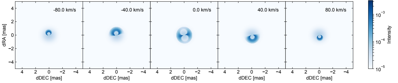
Fig. 6. Synthetic model images calculated for our Keplerian accretion disk model for five spectral channels across the Bry line. We use an arbitrary logarithmic colour scale to show the flux distribution with more detail. The parameters for this model can be found in Table 3.
