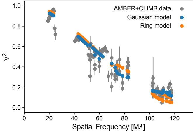
Fig. 2. Visibility squared vs. spatial frequency (baseline length) for our VLT/AMBER and CHARA/CLIMB data for MWC 147. The observed data with uncertainties are shown in grey, whereas the results of our inclined Gaussian and ring models are shown in blue and orange, respectively.
