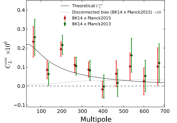
Figure 5. Lensing-mass power spectrum, C_L^{\kappa\kappa} = L^4 C_L^{\phi\phi} / 4 , estimated from the cross-spectrum between BK14 and Planck 2015 data compared with that between BK14 and Planck 2013 data. We also show the theoretical expectation of the disconnected bias in the cross-spectrum between the BK14 and Planck 2015 data multiplied by 10. The cross-spectrum between BK14 and Planck 2013 is offset in L for clarity.
