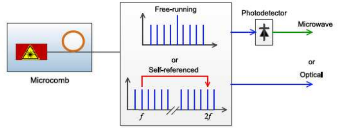
Fig. 2. Microwave and optical frequency synthesis with a microcomb. A microwave signal can be generated by detecting the beat note of a free-running comb or a self-referenced comb locked to a stable optical reference.
