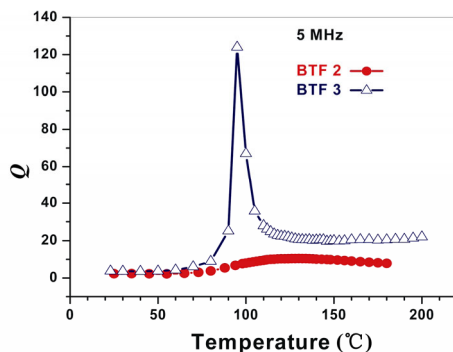
Fig. 11 Changes of Q factor with annealing temperature.
