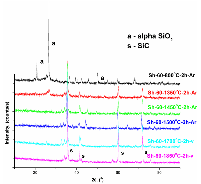
Figure 8. XRD patterns of Sh-60 powder sintered at various temperatures
