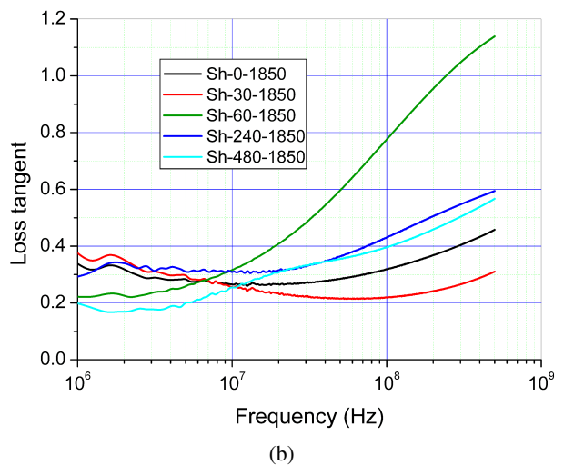
Figure 12. Loss tangent of samples sintered for 2 h at: a) 1700 and b) 1850 °C
