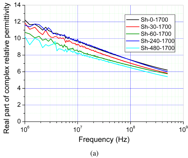
Figure 11. Real part of the complex relative permittivity of samples sintered for 2 h at: a) 1700 and b) 1850 °C
