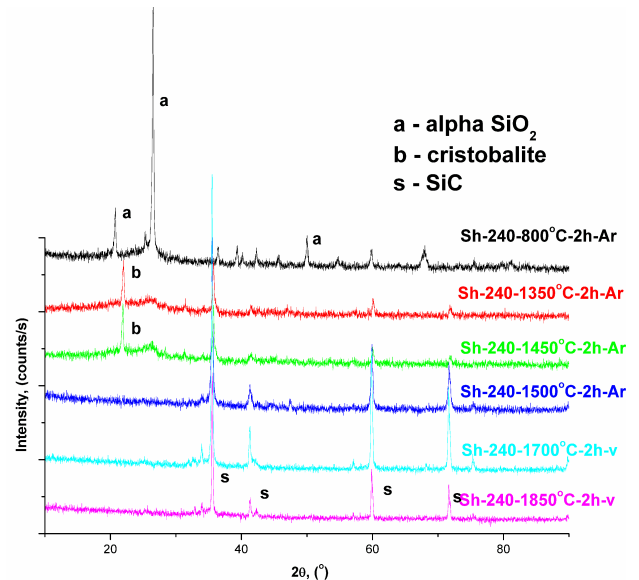
Figure 9. XRD patterns of Sh-240 powder sintered at various temperatures
