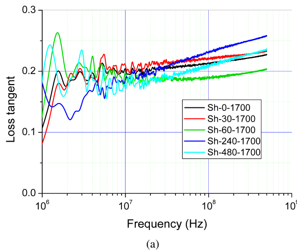
Figure 12. Loss tangent of samples sintered for 2 h at: a) 1700 and b) 1850 °C
