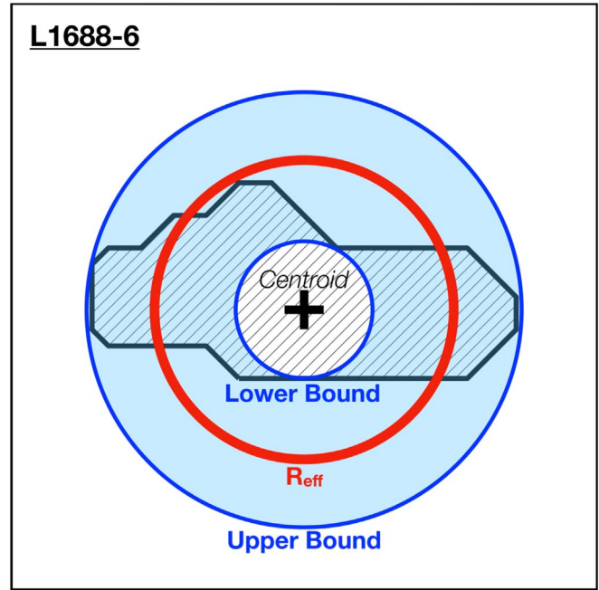
Figure 26. Droplet L1688-d6 as an example of how the lower and the upper bounds of the radius measurement are defined. The droplet is shown as an irregular hatched area. The red circle shows the effective radius, R_{\text{eff}} , derived from the principal component analysis (PCA) weighted by the peak \text{NH}_3 brightness, T_{\text{peak}} (see Section 3.2). The inner blue circle marks the largest circle that can be enclosed by the droplet boundary, which we use as the lower bound in the radius measurement. The outer blue circle marks the smallest circle that can enclose the droplet boundary, which we use as the upper bound in the radius measurement. Notice that the circles used in determining the lower and upper bounds are required to center at the position centroid of the droplet (the positions listed in Table 1).
