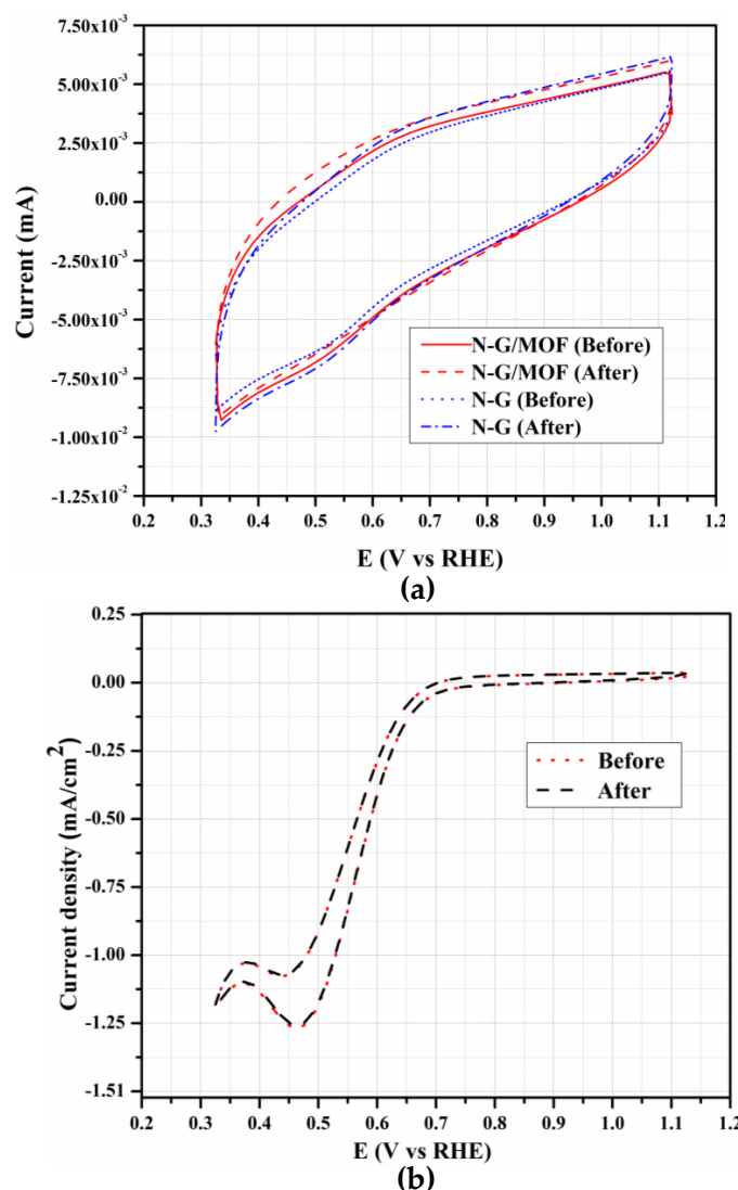
Figure 5. (a) Potential cycling durability study of N-G and N-G/MOF catalysts in nitrogen saturated conditions, and (b) cyclic voltammogram ( O_2 saturated 0.1 M KOH) of N-G/MOF catalyst before and after higher oxidation potentials.
