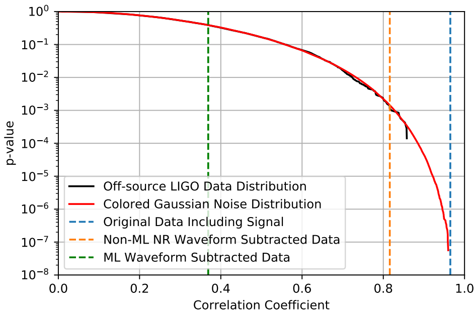
Figure 3. Cumulative distribution of correlations in simulated colored Gaussian noise and detector data away from GW150914, using the same bandpass and notching, and correlation time window settings as used to produce figure 2. The minimum correlation values near the time of flight difference in figure 2 are plotted as vertical lines for reference.
