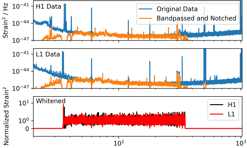
Figure 6. The power spectral density of the data before and after applying the band-pass and notching procedure, used to produce figure 1 of ref. [3]. It is apparent that not all of the spectral lines are removed by the simple choices made to produce figure 1 of ref. [3]. The power spectral density after applying the whitening procedure employed in this section is also shown for comparison. The remaining peak in the power spectral density of the whitened data is due to incomplete down-weighting of the c
