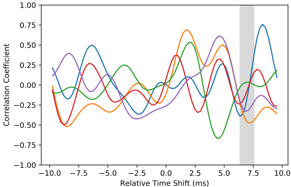
Figure 4. Five examples drawn at random from simulations of uncorrelated colored Gaussian noise. The same grey shaded region as figure 1 is shown. This is the same region that is used to produce the curves plotted in figure 3.
