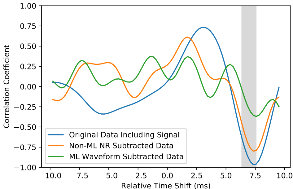
Figure 2. Correlations between the Hanford and Livingston data released at ref. [5] that has been bandpassed and notched in the same way as used to produce figure 1 of ref. [3]. This data has an updated calibration compared to data used in ref. [3]. Therefore the orange and blue curves are not exactly identical (although very similar) to those plotted in figure 1. The figure also contains the correlations for residuals constructed by subtracting the maximum likelihood model waveform found in refs. [21, 22]. The correlations for these residuals are seen to be significantly lower than for the residuals constructed from the example numerical waveform from figure 1 of ref. [3].
