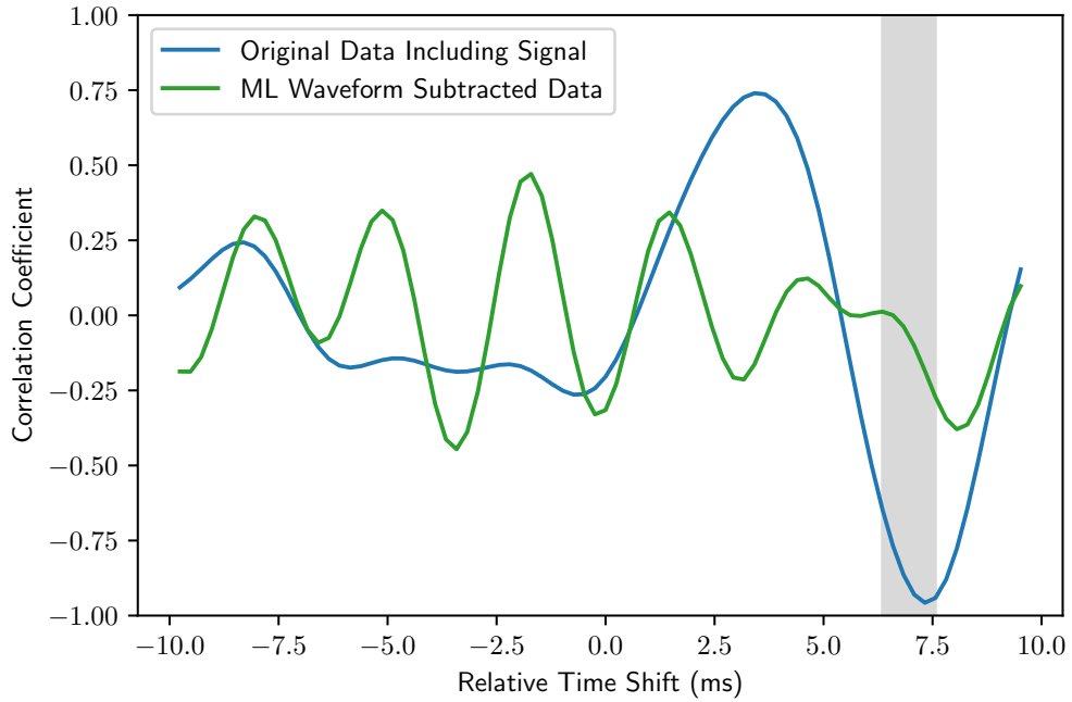
Figure 7. Correlations of residuals after subtracting the maximum-likelihood model waveform, whitening, and bandpassing from 35–350Hz. The maximum and minimum peaks in the ML residuals (green line) are now away from the time of flight delay of \sim 7 ms.
