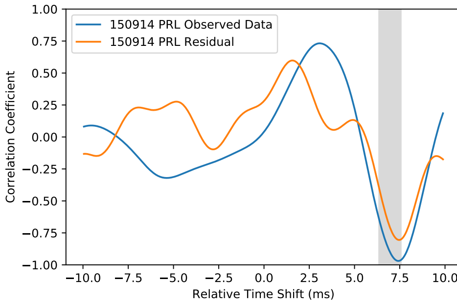
Figure 1. Correlations between timeseries data of the Hanford and Livingston detectors that are displayed in figure 1 of ref. [3]. The correlations shown are for both the data containing the GW150914 signal (in blue) and the example residuals produced after subtracting a numerical relativity GR waveform (in orange). As found in ref. [20] and ref. [2], both the data containing the GW150914 signal and the example residuals show a significant correlation at a time shift corresponding to the time delay between the signal arriving at the Livingston detector and then arriving at the Hanford detector. The grey shaded region shows a region from 6.5 ms to 7.5 ms that contains the time shift between the Hanford and Livingston detectors for the signal observed by LIGO.
