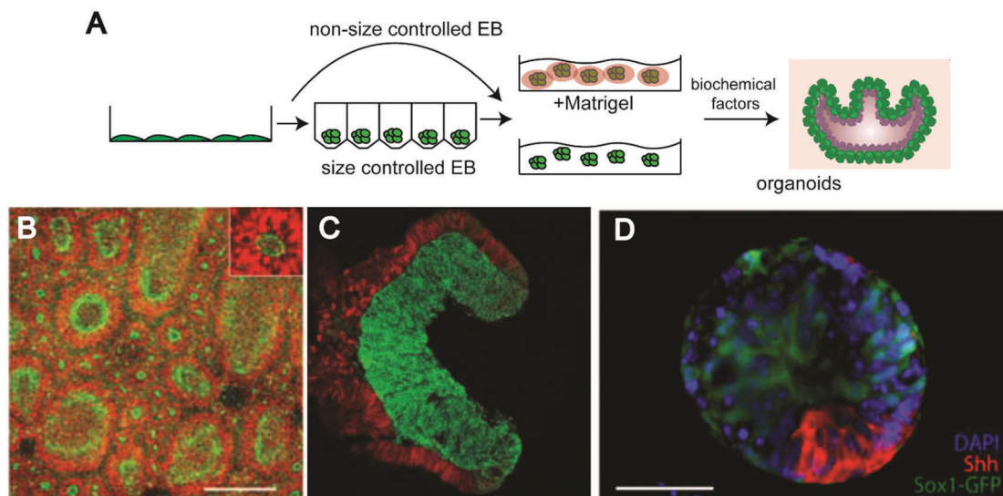
Fig. 1 Self-organized development models. (A) Schematic of methods used in the self-organized development of organotypic cultures. (B) Neural rosettes formation. Cells were stained for Pax6 (red) and N-cadherin (green). The inset shows the magnified structure of a rosette. Scale bar, 100 \mu m. Adapted with permission ref. 22. (C) A two-wall optic cup from derived from mouse embryonic stem cells. Red: Mitf, green: Rx-GFP. Adapted with permission ref. 24. (D) A dorsoventrally polarized neural cyst; red: SHH, green: Sox1, blue: DAPI. Scale bar, 50 \mu m. Reprinted with permission ref. 29.
