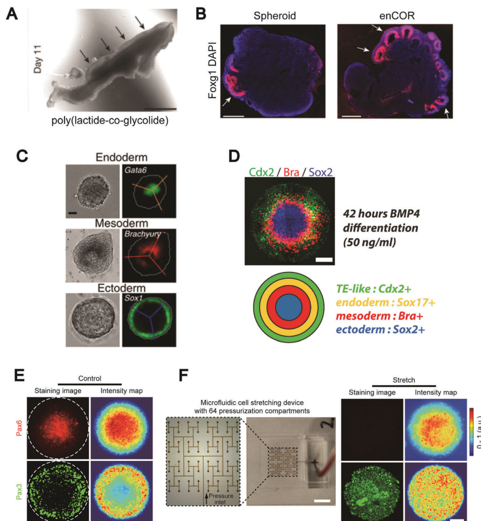
Fig. 2 Engineered development models. (A) Bioengineered EBs from H9 cells at day 11, during neural induction. Arrows mark polarized neural ectoderm. (B) Formation of spheroid cerebral organoids with elongated shapes termed microfilament-engineered cerebral organoids (enCORs). Cells were stained for Foxg1 (red) and nuclear (DAPI, blue). Arrows indicate radial neural epithelium. Adapted with permission ref. 37. (C) Phase and fluorescence images of a differentiated 3D colony. Scale bar, 50 \mu\text{m} . Adapted with permission ref. 40. (D) Formation of germ layers in vitro as a model of gastrulation. Scale bars, 100 \mu\text{m} . Adapted with permission ref. 63. (E) Developmental patterning of neural ectoderm from geometric confined human ESCs. (F) A custom-designed microfluidic cell stretching device that expands only the central regions of micropatterned human ESCs colonies to enhance cell area and contractile forces in situ , we found activation of p-Smad 1/5 upon stretching, and a significant number of NPB cells at colony center. Adapted with permission ref. 71.
