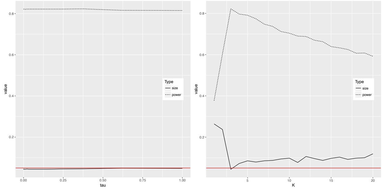
Figure 4: Sensitivity study of power as a function of tuning parameters \tau and K when n = 100 , p = 100 , and K_0 = 3 in the linear regression problem based on 1000 simulations. Dotted and black lines represent empirical power and sizes of the proposed method, while red lines serve as a reference of the nominal size \alpha = .05 .
