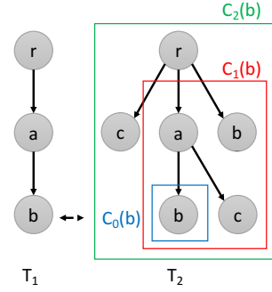
Figure 5: Candidate set C_\alpha(b) for \alpha = 0, 1 and 2 .
