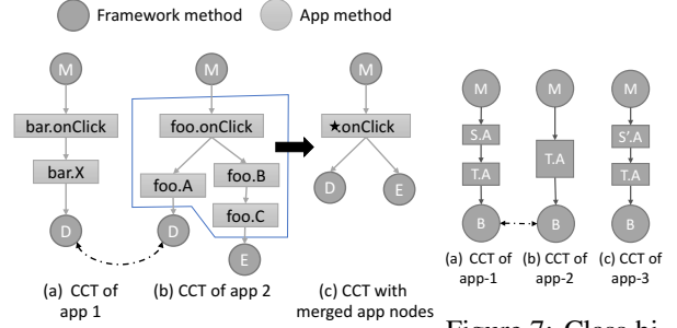
Figure 7: Class hierarchy problem.
