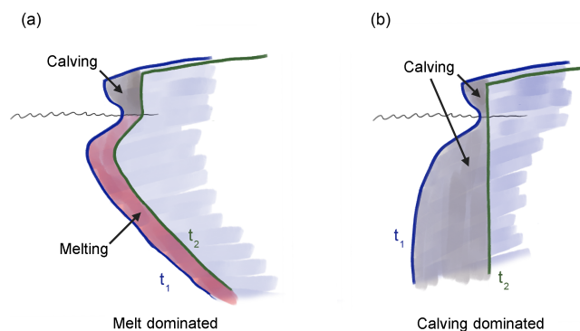
Figure 9. Schematic of two distinct ablation regimes. (a) Melt-dominated regime: the vertical structure of melting due to a rising subglacial discharge plume that entrains warm ambient water results in substantial undercutting of the glacier front (as in profiles A and B in Fig. 8). These front profiles likely do not cause large calving events, with calving mostly confined to the smaller above-water cliff. Profiles are drawn for an earlier time t_1 and a later time t_2 by which the glacier has retreated mostly due to melting. (b) Calving-dominated regime: here the growth of sizable and buoyant underwater feet (as in profiles C and D in Fig. 8) can accelerate calving, with the melt contribution confined to a small region near the water surface. Again, profiles are shown at t_1 and t_2 (pre- and post-calving), as part of the “footloose” calving cycle (Wagner et al., 2014).
