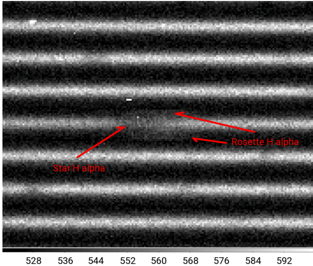
Figure 15. An unprocessed echelle spectrum of GSC 00154–01819. FITS science image 23 has been rotated 90° and transposed so that dispersion is horizontal with wavelength increasing to the right. Higher orders (longer wavelength) are at the top. The region around the H \alpha line in the 87th order is shown. The vertical dimension is angular displacement from the star, and the background Rosette nebula contributes at a greater radial velocity than the star's.
