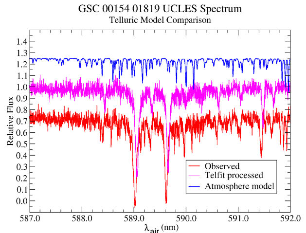
Figure 4. The Na D line region of the spectrum of GSC 00154–01819 from Telfit processing. The observed spectrum, a telluric best-fitting model, and the cleaned spectrum with telluric lines removed are shown displaced for clarity.
