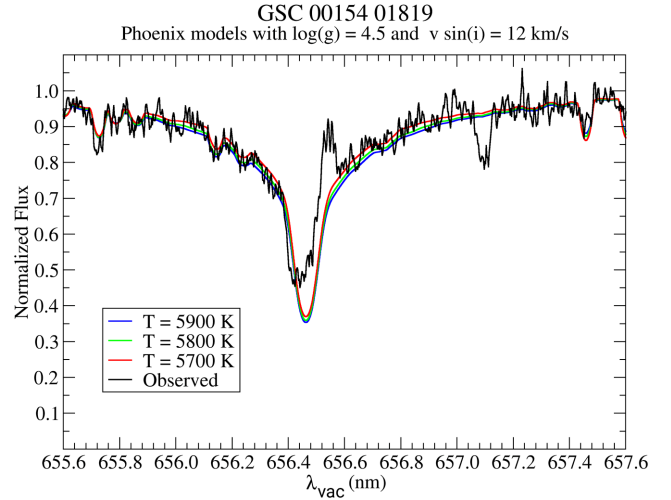
Figure 9. The spectrum of GSC 00154–01819 with telluric lines removed in the region of the H\alpha line compared to rotationally broadened PHOENIX models. Emission on the red side of H\alpha is from H I in the background Rosette nebula. The line at 657 nm is an Fe I 3d^7 4p-4d transition missing in the PHOENIX models.
