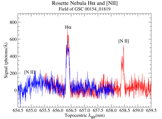
Figure 16. H \alpha and [N II] in the Rosette nebula behind the foreground star GSC 00154–01819. Wavelengths shown are in air for the date and time of observation, calibrated by Telfit. The signal shown is for an effective aperture of 0.32 arcsec 2 with a total of 3600 s exposure time.
