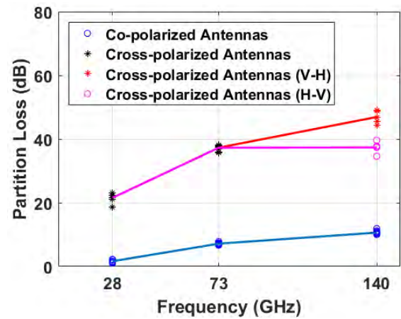
FIGURE 12. Partition loss measurement results of clear glass with a thickness of 1.2 cm at 28, 73, and 140 GHz. Partition loss trends to increase with frequencies for both co-polarized and cross-polarized antenna configurations.
