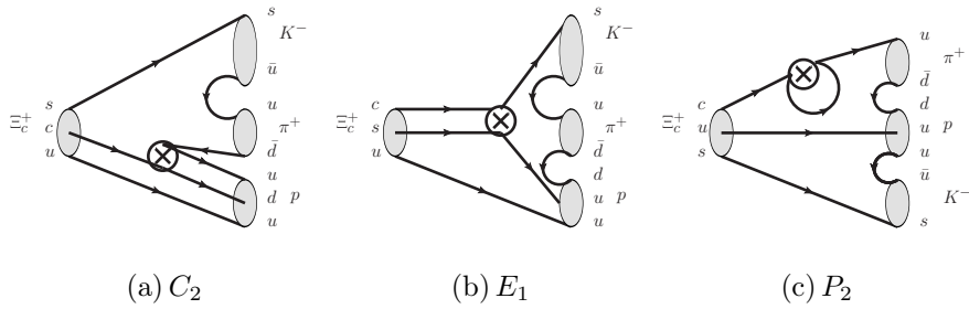
FIG. 4. Diagrams in \mathcal{A}(\Xi_c^+ \rightarrow p K^- \pi^+) = (-\Sigma + \Delta)(-C_2) + (\Sigma + \Delta)(-E_1) + \Delta(-P_2) .
