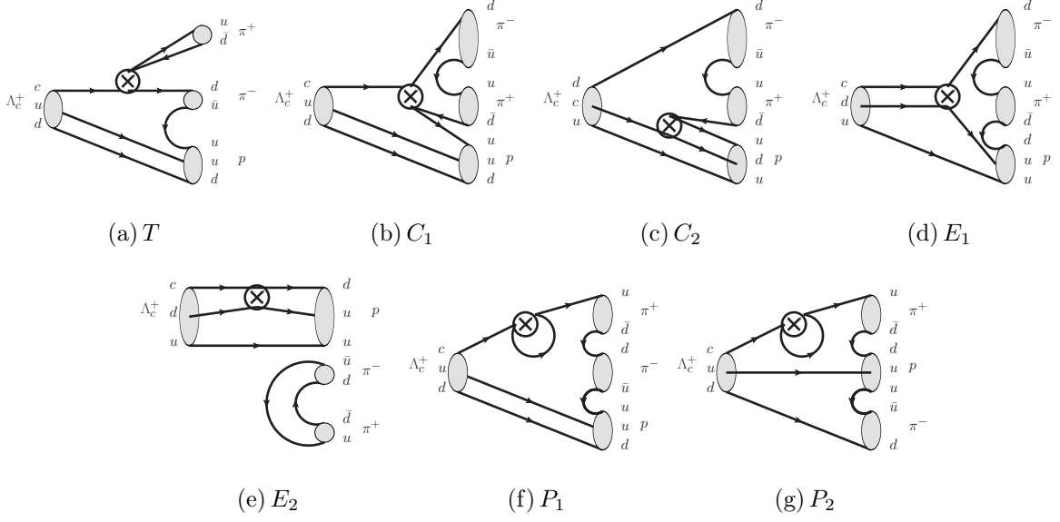
FIG. 5. Diagrams in \mathcal{A}(\Lambda_c^+ \rightarrow p\pi^-\pi^+) = (-\Sigma + \Delta)(-T - C_1 - C_2 - E_1 - E_2) + \Delta(-P_1 - P_2) .
