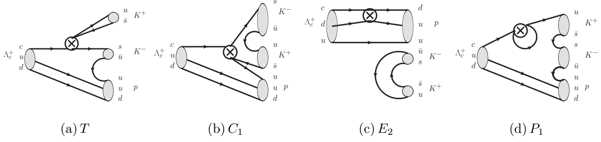
FIG. 1. Diagrams in \mathcal{A}(\Lambda_c^+ \rightarrow p K^- K^+) = (\Sigma + \Delta)(-T - C_1) + (-\Sigma + \Delta)(-E_2) + \Delta(-P_1) . All diagrams have been drawn using JaxoDraw [75, 76].
