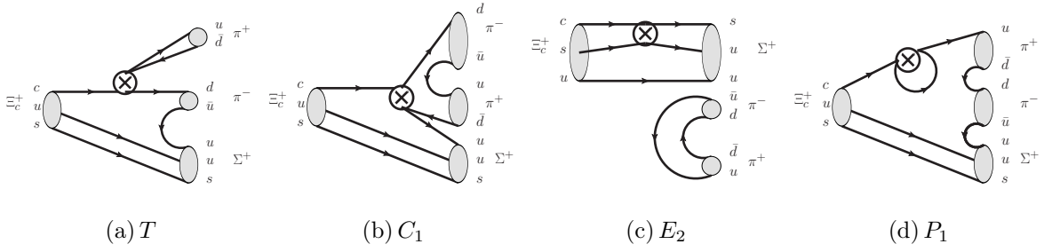
FIG. 2. Diagrams in \mathcal{A}(\Xi_c^+ \rightarrow \Sigma^+ \pi^- \pi^+) = (-\Sigma + \Delta)(-T - C_1) + (\Sigma + \Delta)(-E_2) + \Delta(-P_1) .
