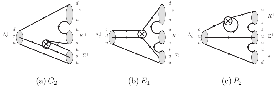
FIG. 3. Diagrams in \mathcal{A}(\Lambda_c^+ \rightarrow \Sigma^+ \pi^- K^+) = (\Sigma + \Delta)(-C_2) + (-\Sigma + \Delta)(-E_1) + \Delta(-P_2) .
