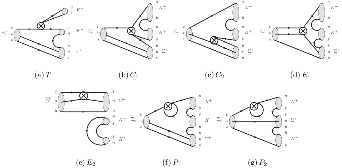
FIG. 6. Diagrams in \mathcal{A}(\Xi_c^+ \rightarrow \Sigma^+ K^- K^+) = (\Sigma + \Delta)(-T - C_1 - C_2 - E_1 - E_2) + \Delta(-P_1 - P_2) .
