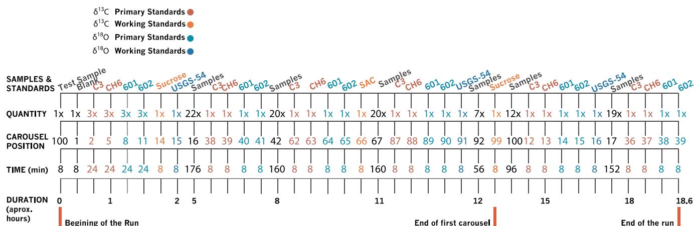
Fig. 7. Sketch showing the sequence of standards and samples for a single run of the HTP procedure of the dual measurement of \delta^{18}\text{O} and \delta^{13}\text{C} ratios implemented at LDEO. The quantity, numbered position in the carousel and length of the analysis time per sample in minutes are indicated below the type of sample. An overall timeline (in hours) for a complete run before a cleaning cycle is indicated on the bottom. Note that the carousel has 100 holes and that each measurement takes about 8 min, considering the time needed to run three peaks of CO reference gas before each sample and one peak of CO gas after the sample. In total, a complete run consists of 100 sample and 39 standard measurements over an 18.6-hour period.
