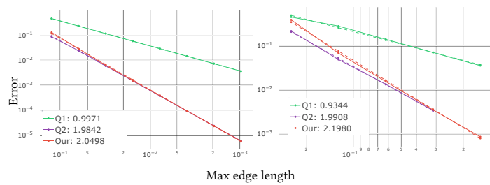
Fig. 19. Poisson equation convergence plot in H_1 norm on a regular grid in 2D (first plot) and 3D (second plot).
