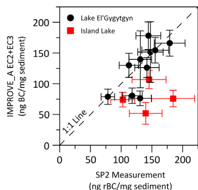
Fig. 6. Comparison of independent SP2 and IMPROVE_A (EC2 + EC3 fractions) measurements of BC for Lake El'Gygytgyn ( n = 10 ) and Island Lake ( n = 4 ) samples. Vertical error bars represent uncertainties from the IMPROVE_A method derived from replicate analyses and the minimum detection limit (Chow et al. 2007). Horizontal error bars represent the relative percentage difference of method replicates from the SP2 measurements. The IMPROVE_A method underestimated BC relative to SP2 measurements at island Lake.
