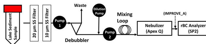
Fig. 1. Schematic of the sample introduction system for lake sediment samples. Dashed arrow denoted by (IMPROVE_A) indicates where a quartz fiber filter was inserted to capture aerosol for independent method verification.
