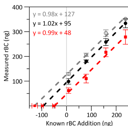
Fig. 3. Standard addition experiments demonstrate no matrix effects. Shown are results for two samples from Lake El'Gygytgyn (gray, black) and one sample from Island Lake (red) using the rBC-like material Aquadag as the standard. Red points on the x-axis represent sample measurements without standard addition. Error bars represent \pm 1\sigma ( n = 3 for all points).
