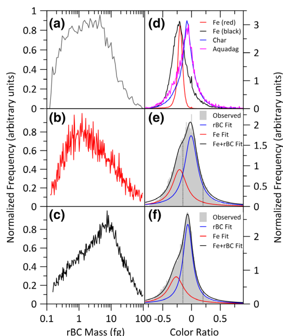
Fig. 2. rBC mass distribution for Aquadag (a), Island Lake (b), and Lake El'Gygytyn (c) samples using equal-width bins in log-space with 20 \mu\text{m} inline filter. Mass distributions are comparable to those reported for rBC in mid-latitude snow and rainwater (Ohata et al. 2013; Schwarz et al. 2013; Wendl et al. 2014) and remained unchanged using 10 and 2 \mu\text{m} inline filters. Color ratios for rBC (Aquadag, char) and iron oxide (i.e., hematite) reference materials (d). Observed (gray) and fit (black) color ratios for Island Lake (e) and Lake El'Gygytyn (f). Fit was calculated as the sum of Cauchy distributions for rBC (blue) and interference (red) portions of the observed color ratio. Only particles with color ratios between the dashed vertical lines at -0.15 and 0.2 were kept in post-processing and used for mass concentration calculations.
