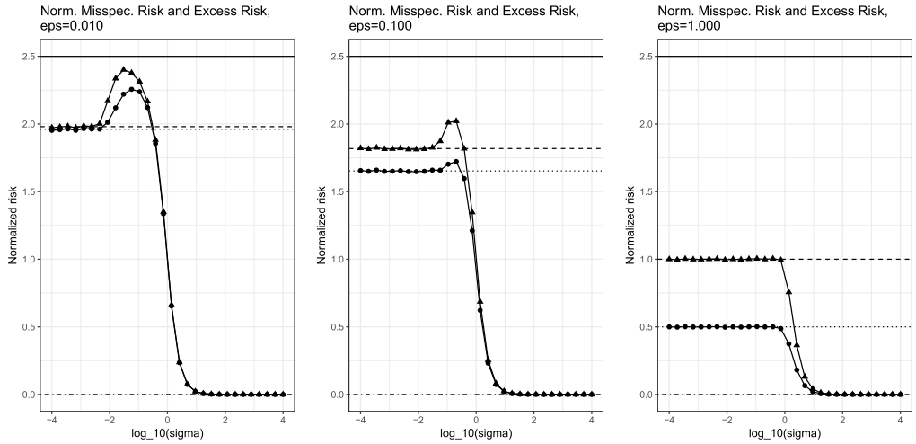
Figure 2. Empirical estimates of the normalized misspecified risk (●) and normalized excess risk (▲) plotted against \log_{10}(\sigma) , for the ball \mathcal{C} = \{\theta \in \mathbb{R}^n : \|\theta\| \leq 1\} in the case n = 3 with \theta^* = (1 + \epsilon, 0, 0) and \epsilon \in \{0.01, 0.1, 1\} . The solid horizontal line represents the upper bound \delta(T_{\mathcal{C}}(\Pi_{\mathcal{C}}(\theta^*))) = n - \frac{1}{2} = 2.5 guaranteed by (7). The dotted lines and dashed lines are the predicted low \sigma limits \frac{n-1}{(1+\epsilon)^2} and \frac{n-1}{1+\epsilon} , respectively. The dash-dot line is the high \sigma limit 0.
