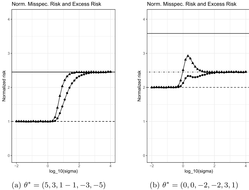
Figure 4. Empirical estimates of the normalized misspecified risk (●) and normalized excess risk (▲) plotted against \log_{10}(\sigma) , for the monotone cone \mathcal{C} = \mathcal{S}^n in the case n = 6 , for two different values of \theta^* . The solid horizontal lines represent the upper bound \delta(T_{\mathcal{C}}(\Pi_{\mathcal{C}}(\theta^*))) guaranteed by (7), which are \delta(\mathcal{S}^6) = H_6 = 2.45 and \delta(\mathcal{S}^4 \times \mathcal{S}^2) = H_4 + H_2 = 3.58\bar{3} , respectively. The dashed lines are the predicted low \sigma limits, which are 1 and 2, respectively. (See Section 4.2 for details on the computations.) The dash-dot line is the predicted high \sigma limit \delta(\mathcal{S}^6) = H_6 = 2.45 (see discussion below Corollary 5.4).
