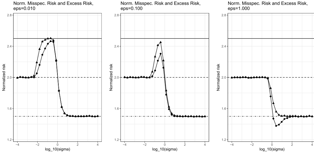
Figure 5. Empirical estimates of the normalized misspecified risk (●) and normalized excess risk (▲) plotted against \log_{10}(\sigma) , for the orthant \mathcal{C} := \mathbb{R}^3_+ and \theta^* = (1, 1, -\epsilon) with \epsilon \in \{0.01, 0.1, 1\} . The solid horizontal line represents the upper bound \delta(T_{\mathcal{C}}(\Pi_{\mathcal{C}}(\theta^*))) = n - \frac{1}{2} guaranteed by (7). The dashed line is the common low \sigma limit n - 1 (see Corollary 4.1). The dash-dot line is the high \sigma limit \delta(\mathbb{R}^n_+) = 3/2 .
