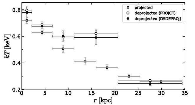
Figure 4. The radial profile of the hot gas temperature in NGC 7049 derived from deprojected (black circles for deprojection with DSDEPROJ and white circles for model project ) and projected spectra (grey squares). To increase the number of counts and mitigate the ringing effect in the deprojection analysis, the spectra from annuli outside the third one were tied by two and thus are displayed as only two points for each deprojection method.
