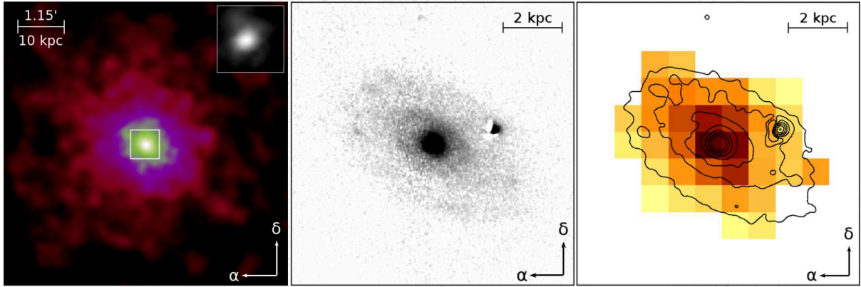
Figure 2. Left: XMM-Newton X-ray (0.3–2.0 keV) image of NGC 7049 composed of data from all EPIC instruments, exposure-corrected and adaptively smoothed. The black-and-white image in the upper-right corner is a detail of the central region observed by the Chandra X-ray Observatory in a 5 ks exposure. Centre: emission of warm ionised gas in H\alpha+[NII] lines observed in NGC 7049 by the SOAR telescope. Right: [CII] line flux obtained by Herschel PACS with contours of the H\alpha+[NII] emission overlaid.
