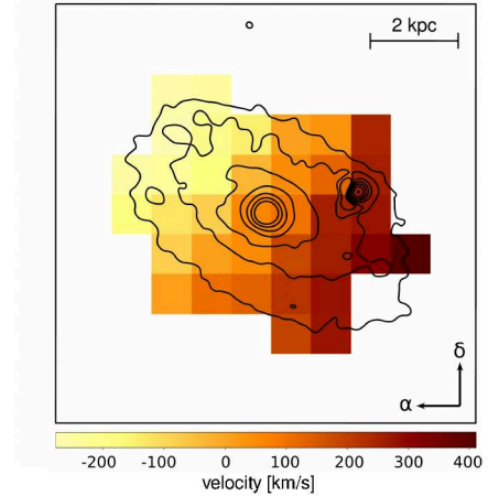
Figure 1. [\text{CII}] line-of-sight velocity map of NGC 7049 based on Werner et al. (2014) . Values are relative to the systemic velocity of the galaxy. The velocity distribution of the [\text{CII}] emitting gas indicates the presence of a disc, rotating with a velocity of v_{\text{rot}} \sim 200\ \text{km s}^{-1} .
