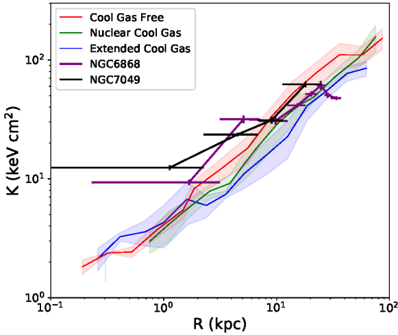
Figure 12. The median entropy profile for a sample of 49 galaxies from Lakhchaura et al. (2018) with the entropy profiles of NGC 7049 and another galaxy with a fast rotating disc of cool gas, NGC 6868, overplotted. The red, green and blue solid lines show median profiles for the cool gas free, nuclear cool gas and extended cool gas systems, respectively and the shaded regions show the median absolute deviation (MAD) spreads about the medians.
