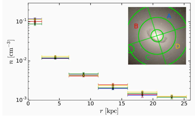
Figure 3. Projected particle densities measured in four directions: red and yellow are approximately parallel with, and blue and green are perpendicular to the plane of rotation of the cold gas disc. For clarity, the disc and the orientation of sectors are shown in a small HST image in the upper right corner.
