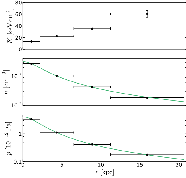
Figure 5. Profile of deprojected entropy K = k_B T n_e^{-2/3} , particle density n and pressure p = nk_B T . The solid green curves are the best-fit \beta -models (see eq. 1 and eq. 2). We note that the errors, especially in the bottom plot, are too small to be visible.
