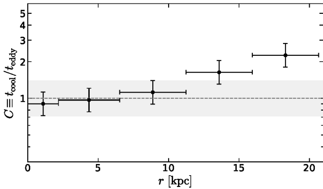
Figure 11. The radial distribution of the cooling time over eddy turnover time for NGC 7049. Grey region represents the 1\text{-}\sigma confidence region (retrieved from hydrodynamical simulations; Gaspari et al. 2018) for significant multiphase condensation to develop.
