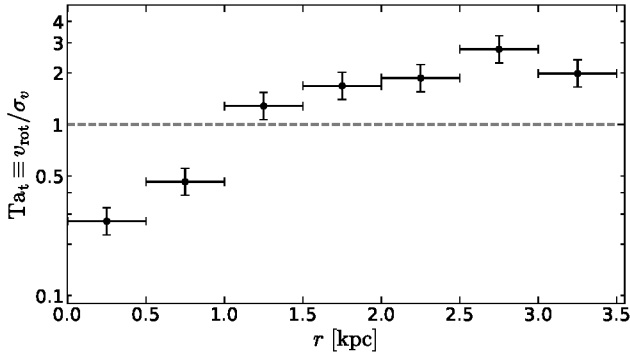
Figure 10. The radial profile of the ratio of rotational velocity and the velocity dispersion for the [CII]-emitting gas. Dashed grey line signifies transition from rotation- to turbulence-dominated dynamics and type of condensation.
