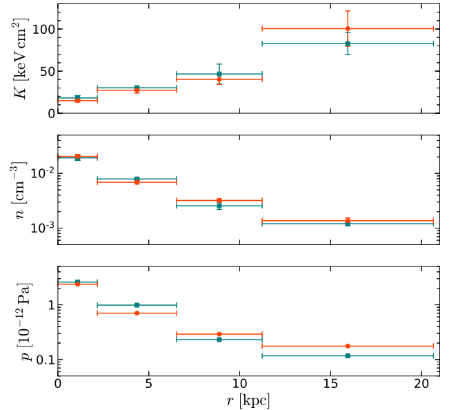
Figure 7. Deprojected profile of entropy K = k_B T n_e^{-2/3} , particle density n and pressure p = nk_B T in sectors along the rotational axis (turquoise squares) and the perpendicular direction (orange dots). We note that errors especially in the bottom plot are too small to be visible.
