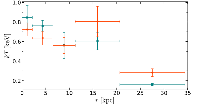
Figure 6. Deprojected temperature profiles determined in sectors along the rotational axis (B+D) and in a perpendicular direction (A+C) shown as turquoise squares and orange dots, respectively.
