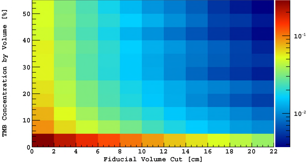
Fig. 95. WIMP-like neutron recoils per year from both U and Th induced by (\alpha, n) reactions in the stainless steel cryostat and in the PTFE panels.
