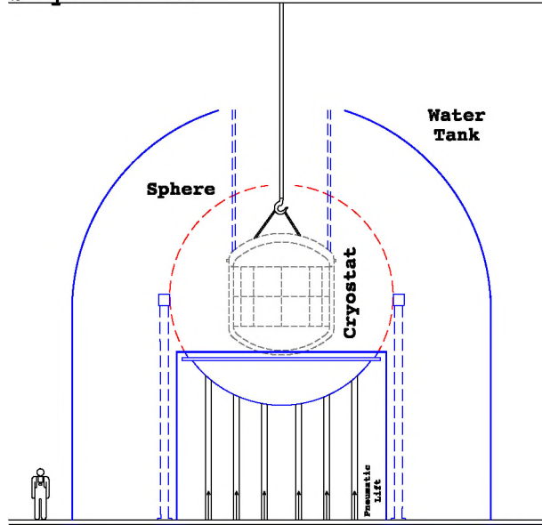
Fig. 86. Schematic drawing of the cryostat installation sequence.
