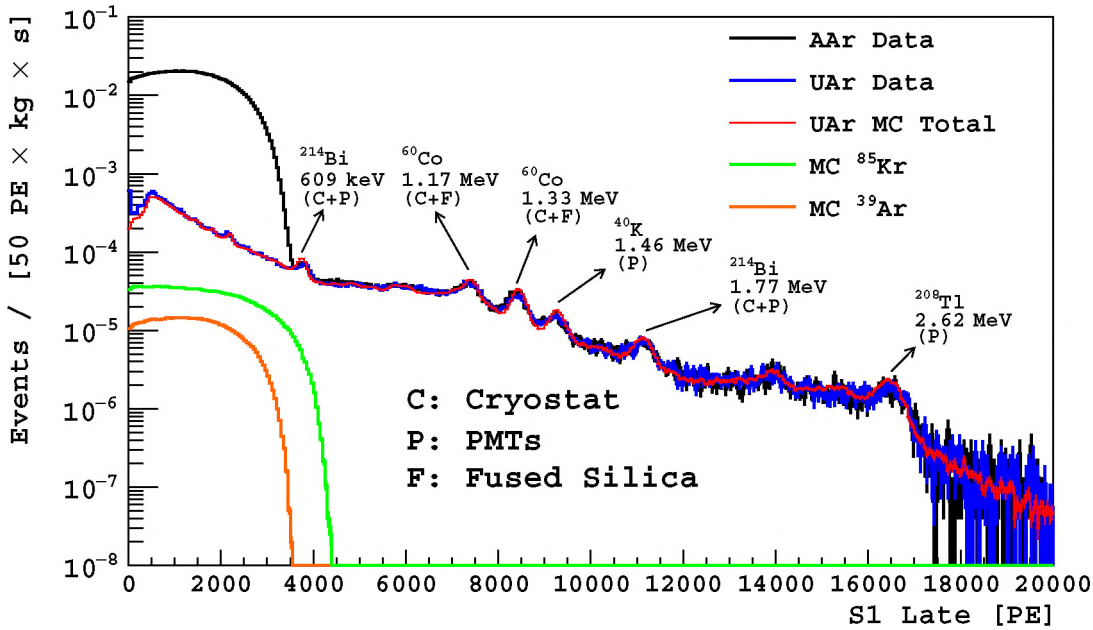
Fig. 90. Comparison of measured field-off spectra for the UAr (blue) and AAr (black) targets, normalized to exposure. Also shown are the G4DS fit to the UAr data (red) and individual components from ^{85}\text{Kr} (green) and ^{39}\text{Ar} (orange) extracted from the fit. S1 Late is a modified S1 variable which begins waveform integration after the first 90 ns, to avoid channel saturation. [72]
