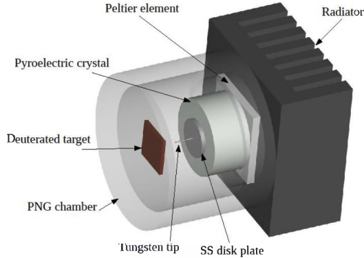
Fig. 64. Pyroelectric neutron generator layout.
