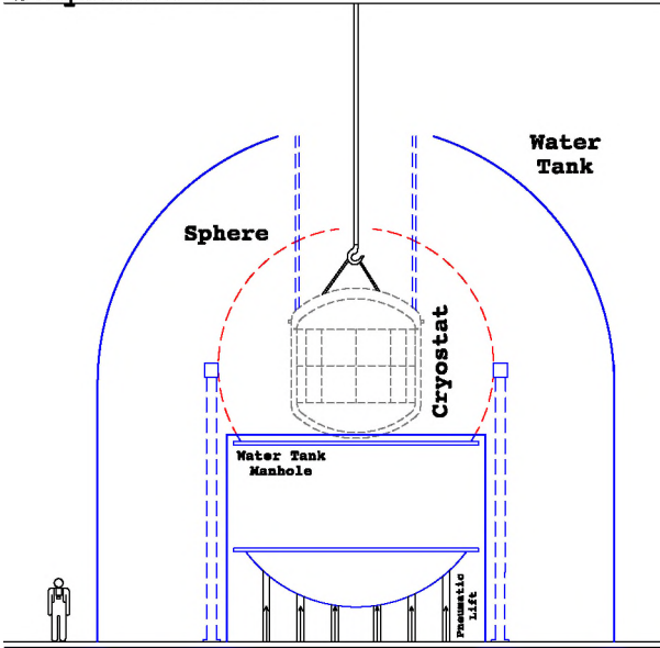
Fig. 86. Schematic drawing of the cryostat installation sequence.
