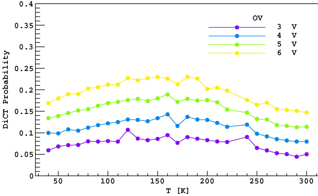
Fig. 27. DiCT probability as function of temperature for different OV for NUV-HD-LF SiPMs. DiCT values exhibit a weak dependence on temperature. [126]
