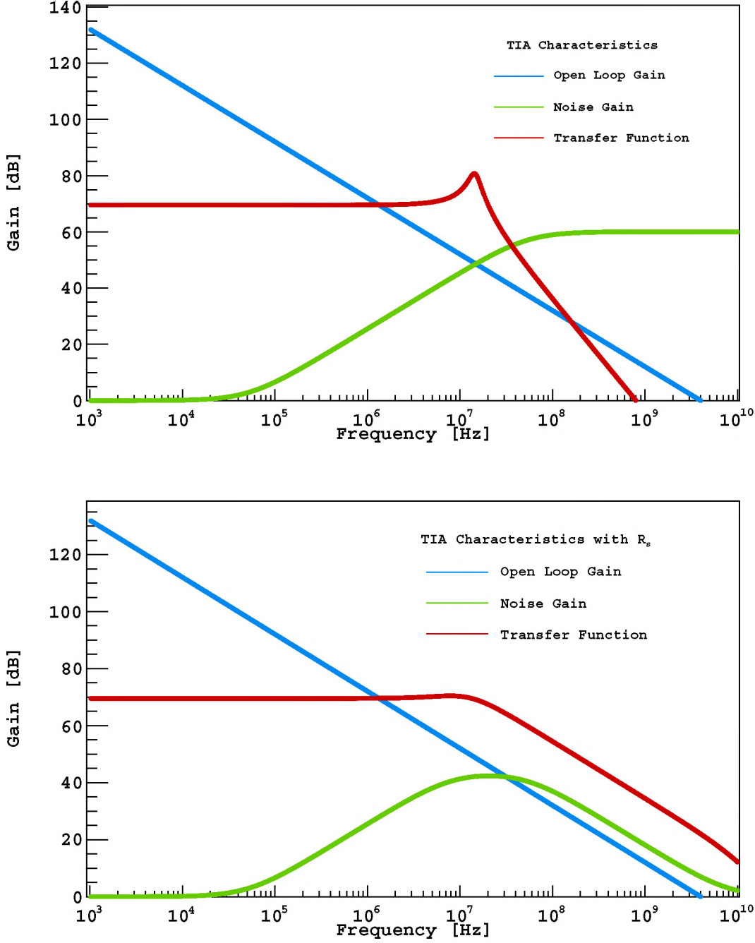
Fig. 30. Top: open loop gain ( A_{Vol} ), noise gain (NG) and transfer Function ( T_z ) of the TIA configured with C_d = 1 \text{ nF} , R_f = 3 \text{ k}\Omega , C_f = 1 \text{ pF} , and R_s = 0 \Omega . Bottom: same distributions with R_s = 20 \Omega .
