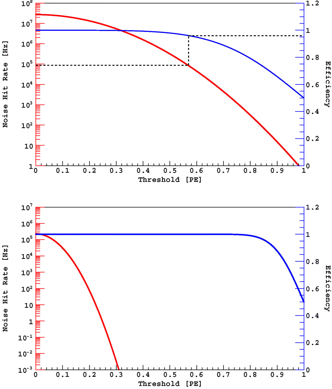
Fig. 36. Top: rate of fake hits above the specified threshold due to electronic noise (in red) and threshold efficiency for real photoelectrons (in blue) for the signal from the TIA + NUV-HD-LF- \text{HR}_q tile of total area of 4 \text{ cm}^2 , corresponding to the left panel of Fig. 35. The dashed line corresponds to a threshold efficiency of 96% with a fake hit noise of 100 kHz. Bottom: same plot with (almost) optimal filter, corresponding to the bottom panel of Fig. 35.
