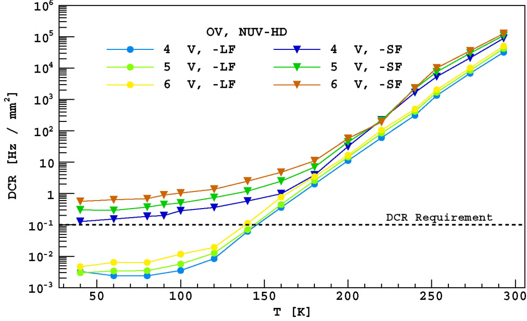
Fig. 25. DCR for NUV-HD-SF (triangular markers) and NUV-HD-LF (circular markers) devices as function of OV and temperature [126].
