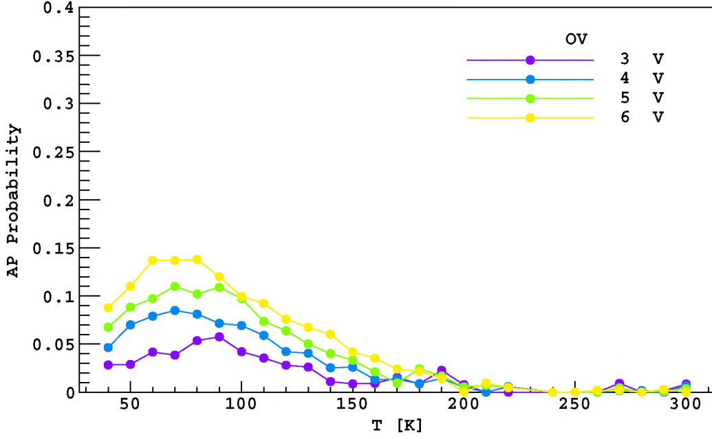
Fig. 26. AP probability as function of temperature for different OV for NUV-HD-LF SiPMs [126].
