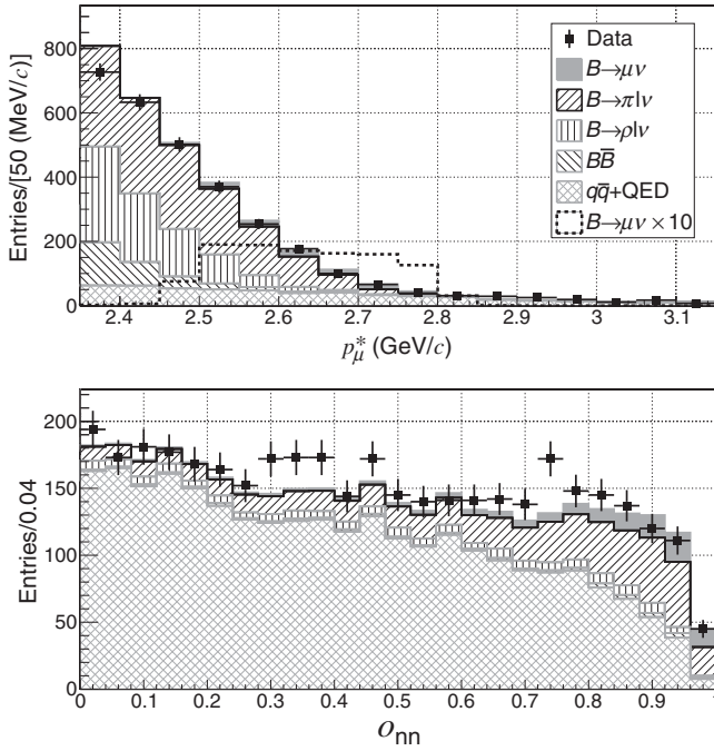
FIG. 2. Projections of the fitted distribution to data onto the histogram axes in the signal-enhanced regions (top panel) 0.84 < o_{nn} and (bottom panel) 2.6 \text{ GeV}/c < p_\mu^* < 2.85 \text{ GeV}/c .
