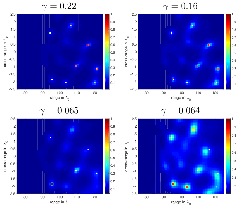
Figure 2. Imaging results using MUSIC with multiple sources and multiple receivers, but a single frequency. \text{SNR} = 0 dB corresponding to additive noise. The scatterers are on the grid. The top left image is obtained using the optimal illuminations, for which \gamma = 0.22 . The other three images are obtained using 12 randomly chosen illuminations, for which the values of \gamma vary.
