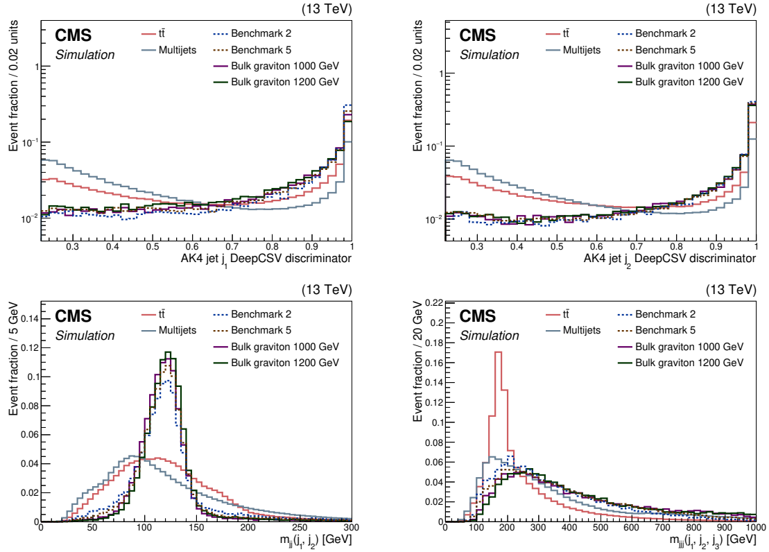
Figure 2. Distributions for AK4 jets of the DeepCSV discriminators for the leading j_1 (upper left) and next leading j_2 (upper right), the invariant mass of j_1 and j_2 , m_{jj}(j_1, j_2) (lower left), and the invariant mass of j_1 , j_2 , and their nearest AK4 jet j_3 , m_{jj}(j_1, j_2, j_3) (lower right), in semi-resolved events. The multijet and t\bar{t} +jets background components are shown separately, along with the simulated signals for bulk gravitons of masses 1000 and 1200 GeV and the non-resonant benchmark models 2 and 5. The distributions are normalized to unity.
