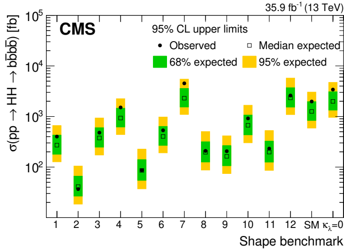
Figure 6. The observed and expected upper limits for non-resonant HH production in the standard model, the model with \kappa_\chi = 0 , and other shape benchmarks (1–12), combining the fully-merged selection and the semi-resolved selection (where the events used in the fully-merged analysis are not considered in the semi-resolved analysis). The inner (green) and the outer (yellow) bands indicate the regions containing the 68 and 95%, respectively, of the distribution of limits expected under the background-only hypothesis.
