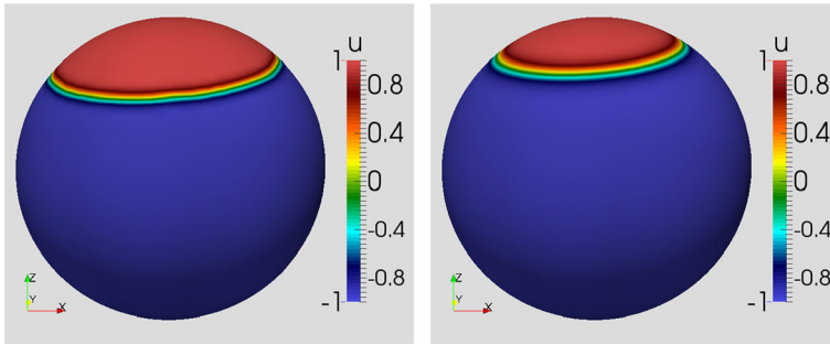
Fig. 2 The shrinking circle at time t = \tau (left) and t = 0.2 (right)
